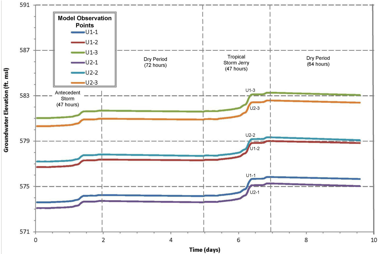
WILLIAM STATES LEE III NUCLEAR STATION UNITS 1 & 2 Maximum Post-Construction Groundwater Analysis, Results Hydrograph FIGURE 2.4.12-211 Rev 7
