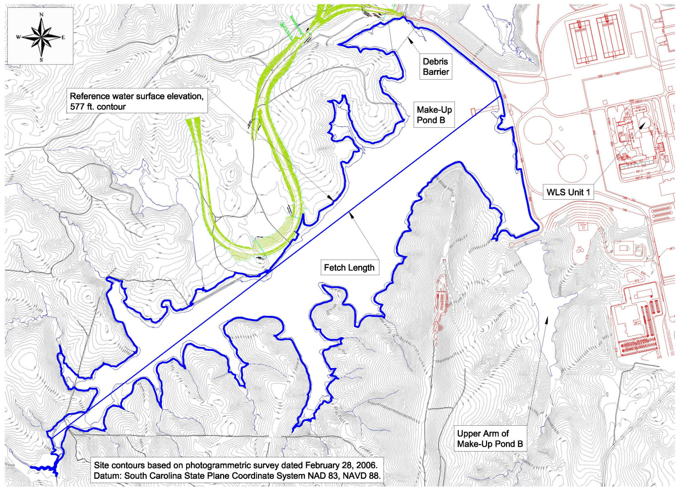
WILLIAM STATES LEE III NUCLEAR STATION UNITS 1 & 2 Make-Up Pond B Extreme Wind Speed Fetch Length FIGURE 2.4.5-202 Rev 7
