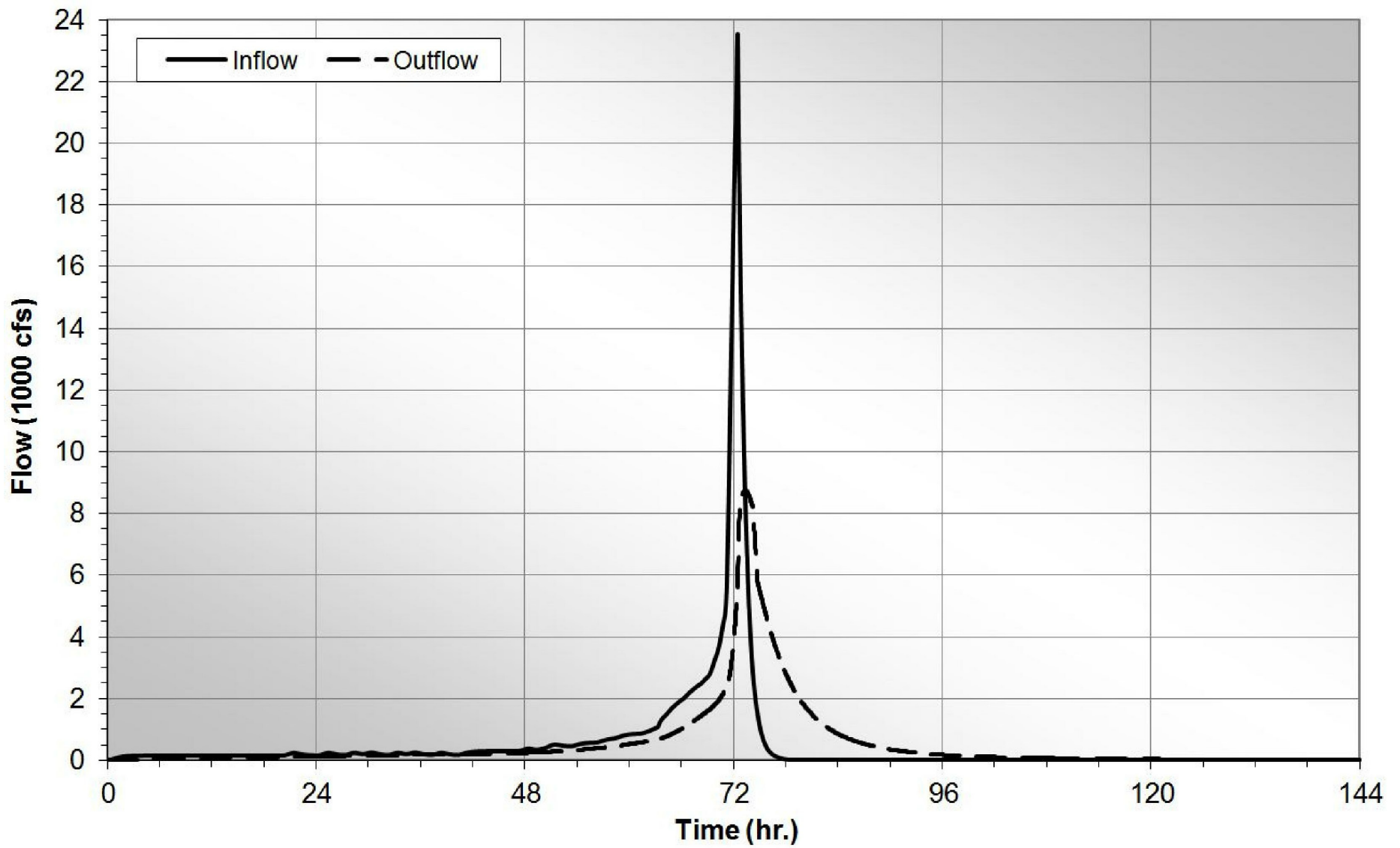
WILLIAM STATES LEE III NUCLEAR STATION UNITS 1 & 2 PMF Hydrograph With Upper Arm Dam Failure, Make-Up Pond B FIGURE 2.4.4-203 Rev 7
