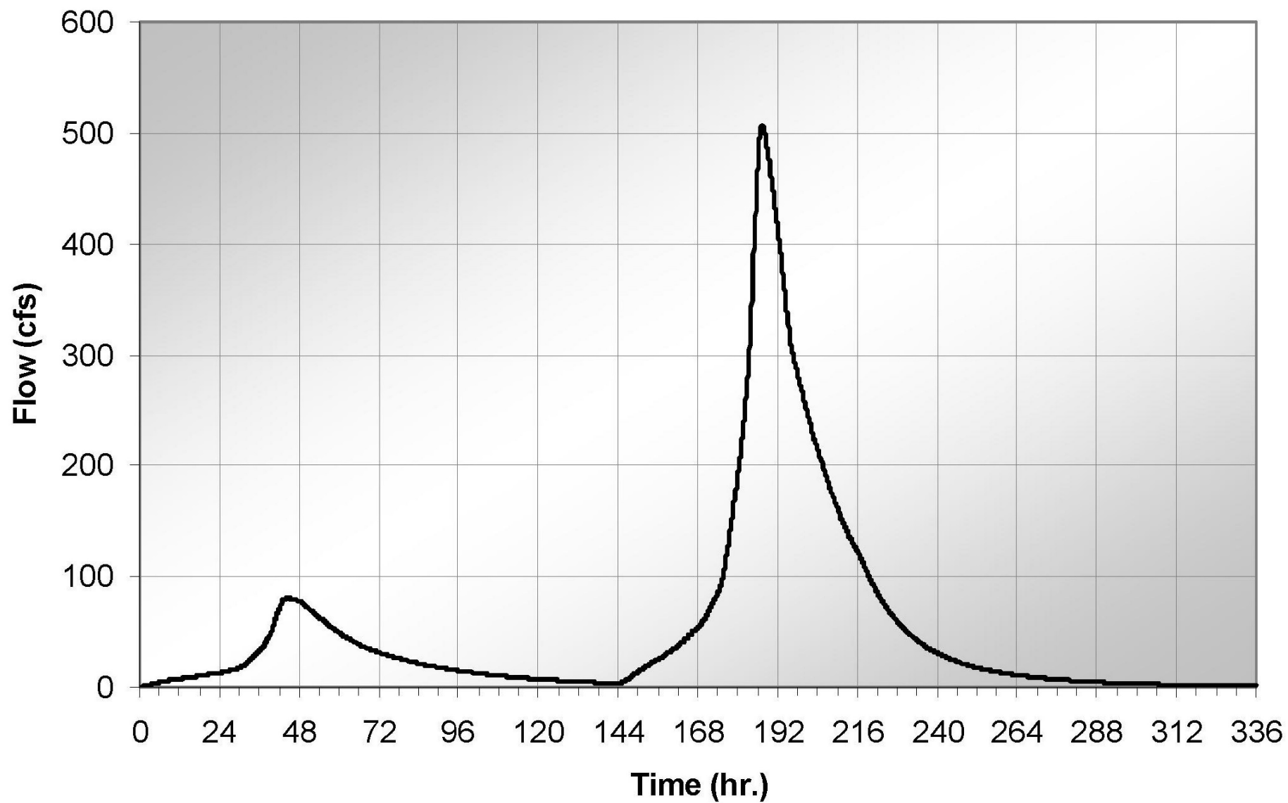
WILLIAM STATES LEE III NUCLEAR STATION UNITS 1 & 2 Subbasin Make-Up Pond C (MUPC) PMF Inflow Hydrograph FIGURE 2.4.3-243 Rev 2
