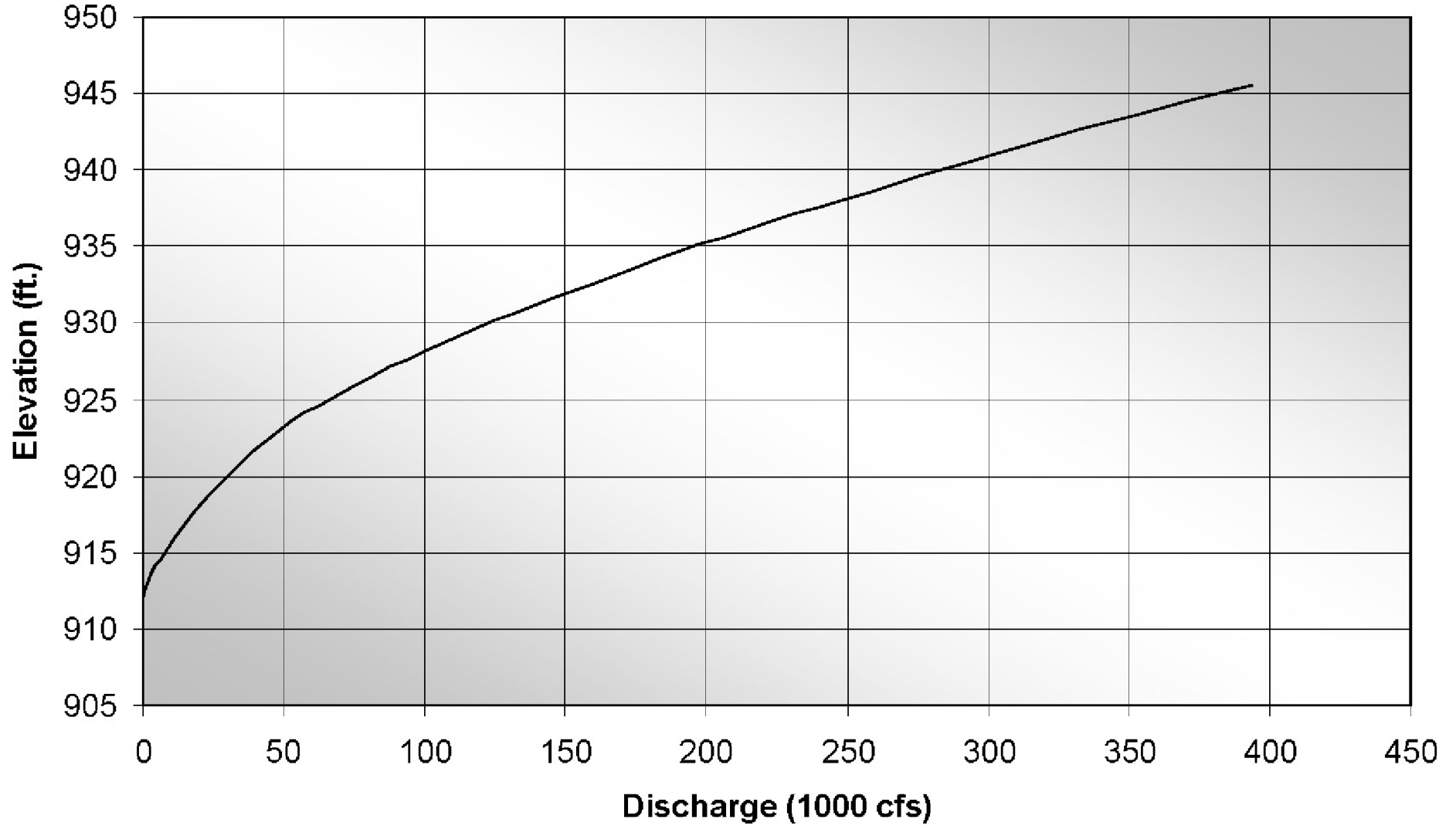
WILLIAM STATES LEE III NUCLEAR STATION UNITS 1 & 2 Discharge Rating Curve, Turner Shoals Dam FIGURE 2.4.3-211 Rev 0
