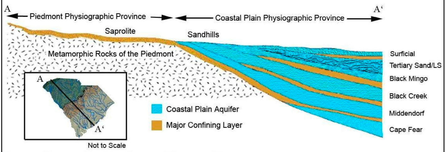
Generalized Hydrogeologic Cross-Section from the Blue Ridge through the Lower Coastal Plain in South Carolina Source: Reference 267
