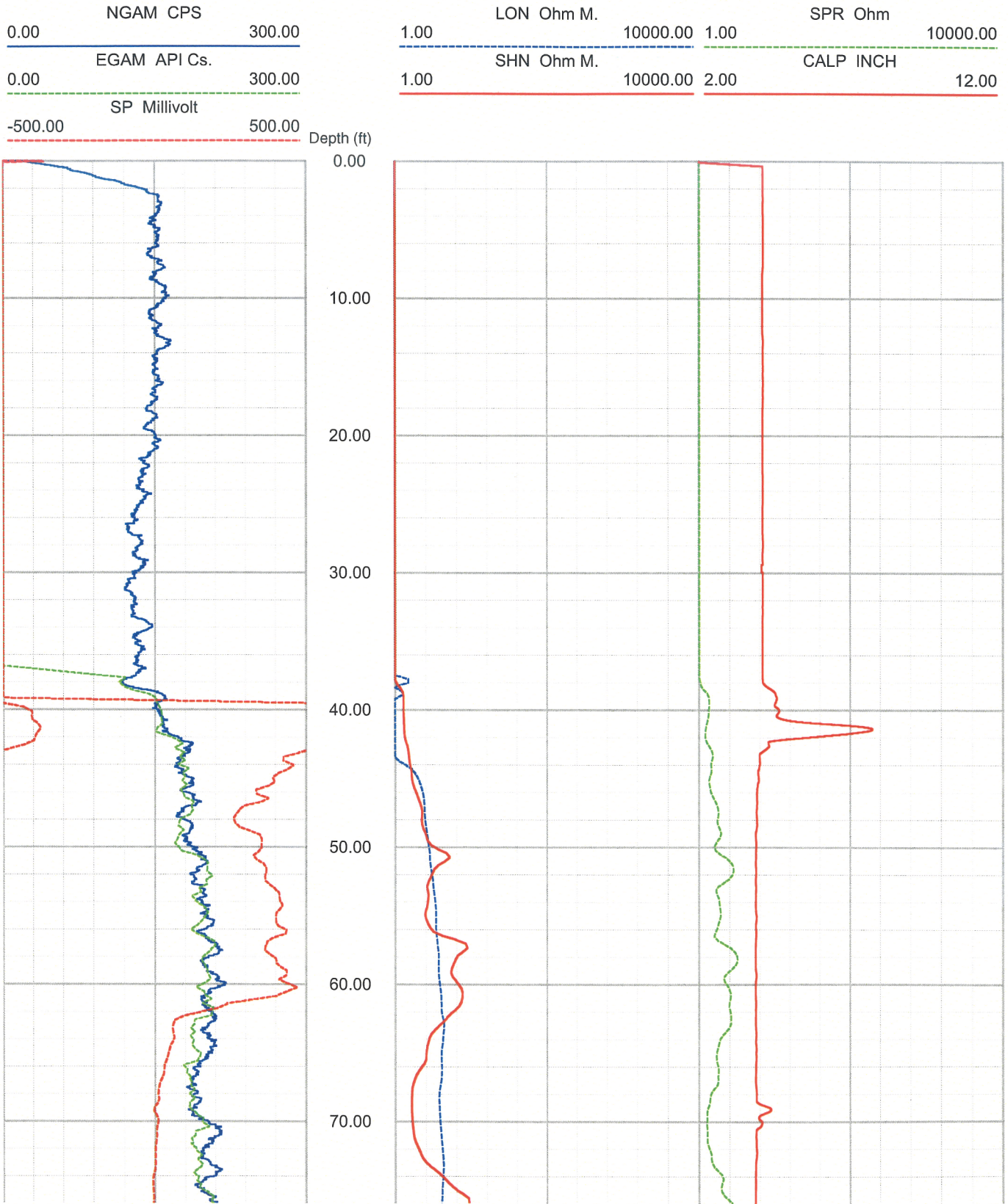
North Anna COL Boring B-901 lower section ELOG, Caliper and Gamma Sheet 2 of 5
