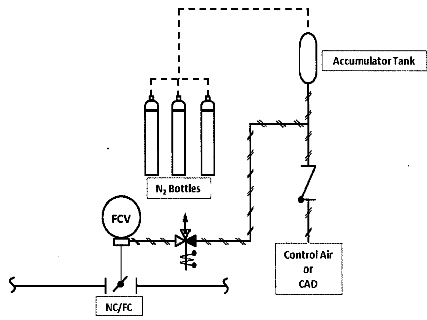
Figure 3 - Typical CIV/FCV Actuator Supply
