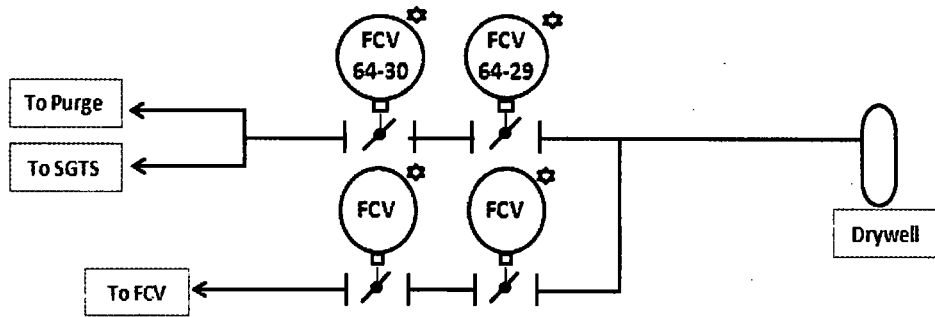
Figure 2 - Drywell Head Vent Detail
