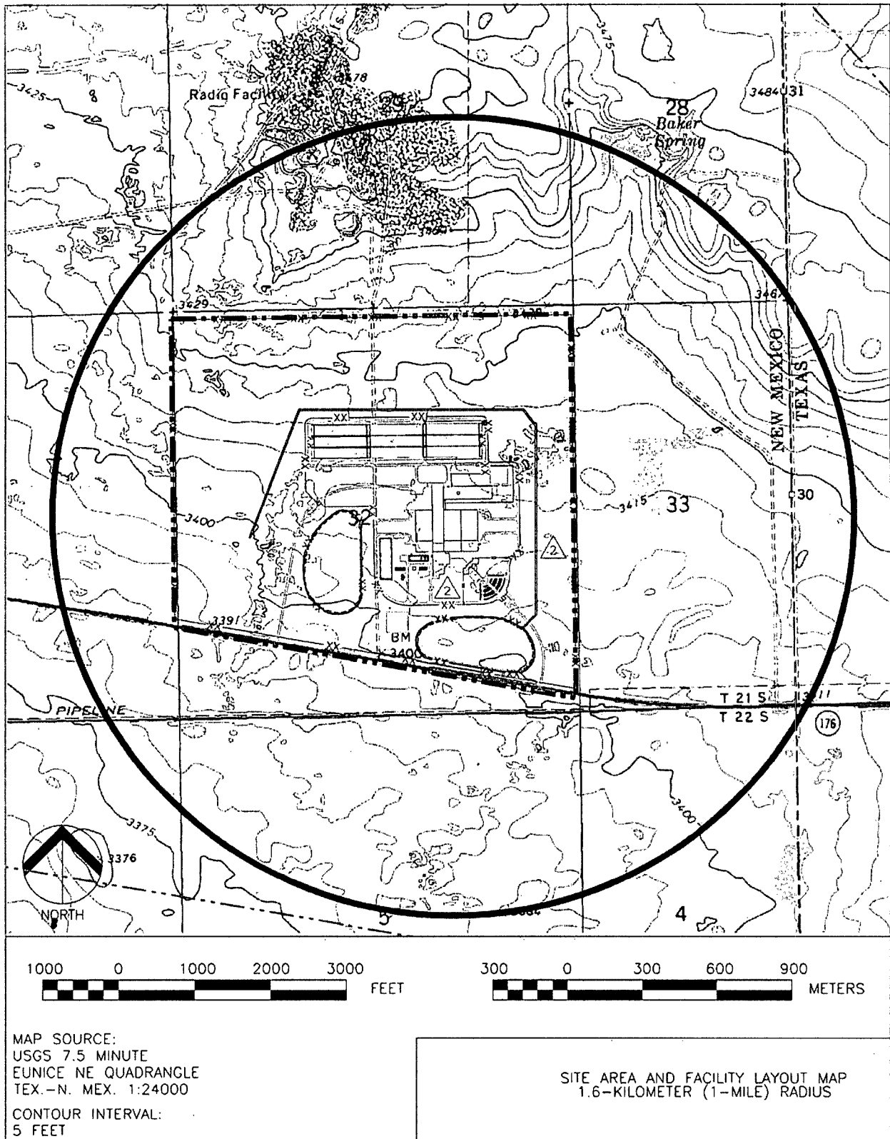
Figure 2.1-2 Site Area and Facility Layout Map 1.6-Kilometer (1-Mile Radius)
