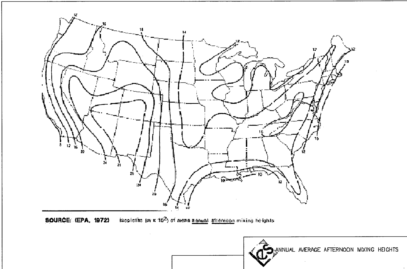
Figure 3.6-9 Annual Average Afternoon Mixing Heights
