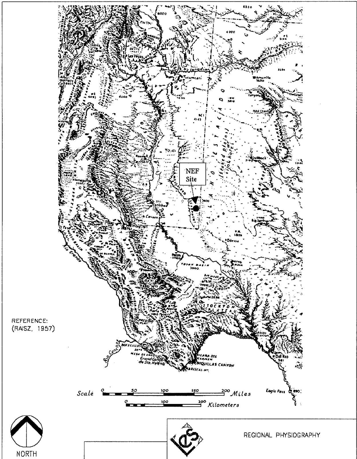
Figure 3.3-1 Regional Physiography
