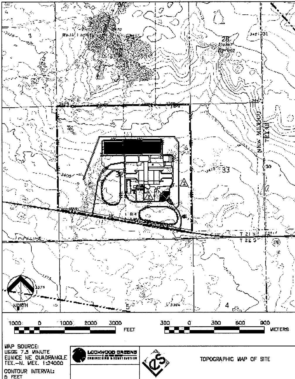
Figure 3.6-11 Topographic Map of Site
