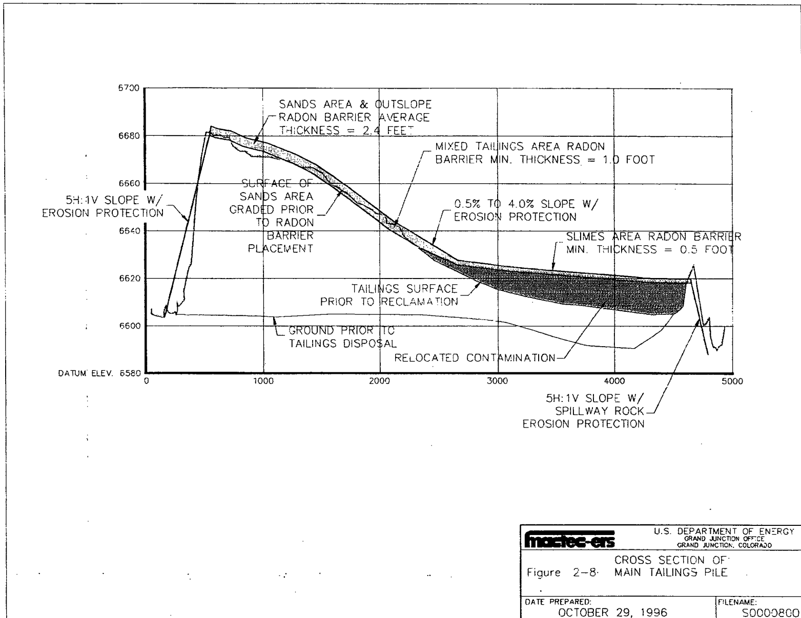
Figure 2-8. Cross Section of Main Tailings Pile
