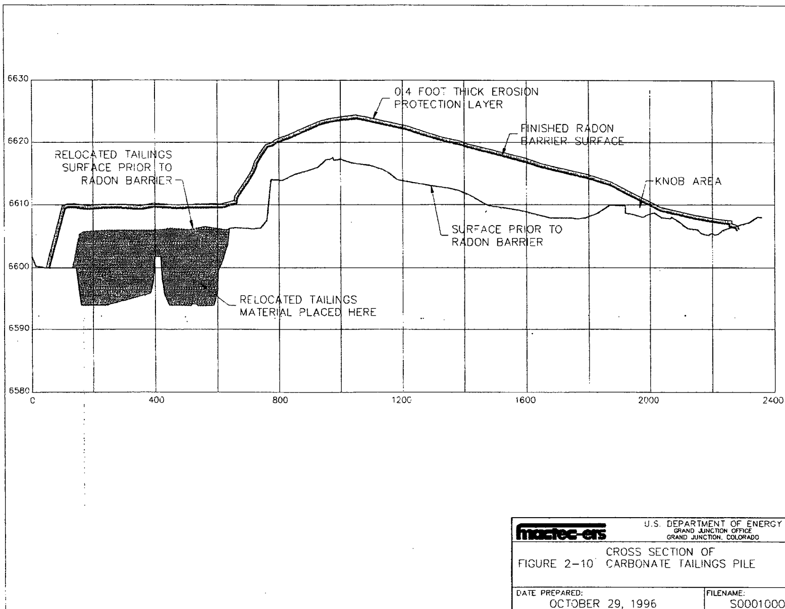
Figure 2-13. Cross Section of Carbonate Tailings Pile
