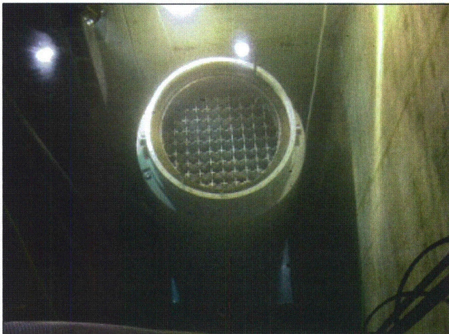
Figure 5: Canister in a Transfer Cask in a Spent Nuclear Fuel Pool
