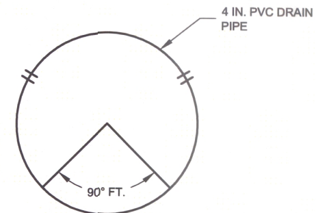
TRENCH BOTTOM SECTION VIEW - PIPE NOT TO SCALE
