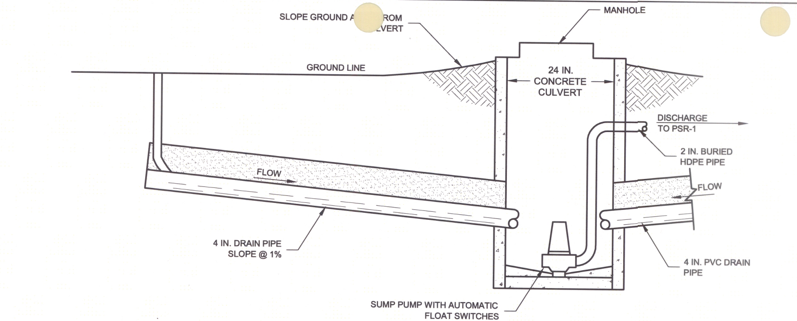
SECTION VIEW - INTERCEPTOR TRENCH NOT TO SCALE
