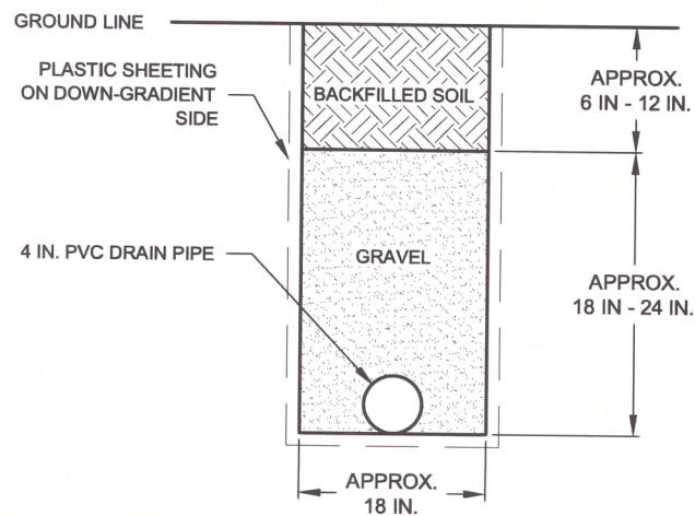
TYPICAL SECTION VIEW - TRENCH NOT TO SCALE
