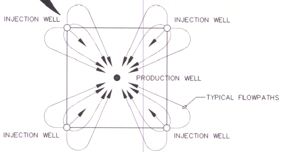
TYPICAL WELLFIELD PATTERN
