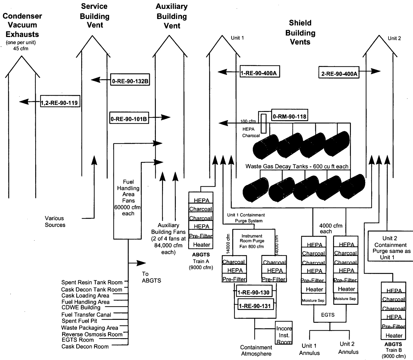
Figure 7.2 - DETAIL OF GASEOUS RELEASE/DISCHARGE POINTS
