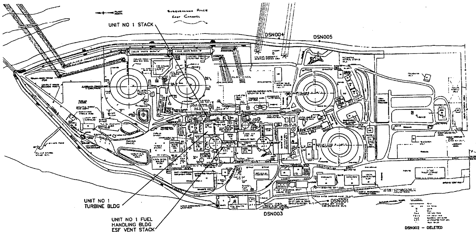
AmerGen Three Mile Island Nuclear Station Gaseous Effluent Release Point and Liquid Effluent Outlet Locations CAD FILE: 6716R16.DWG Fig. 5-3
