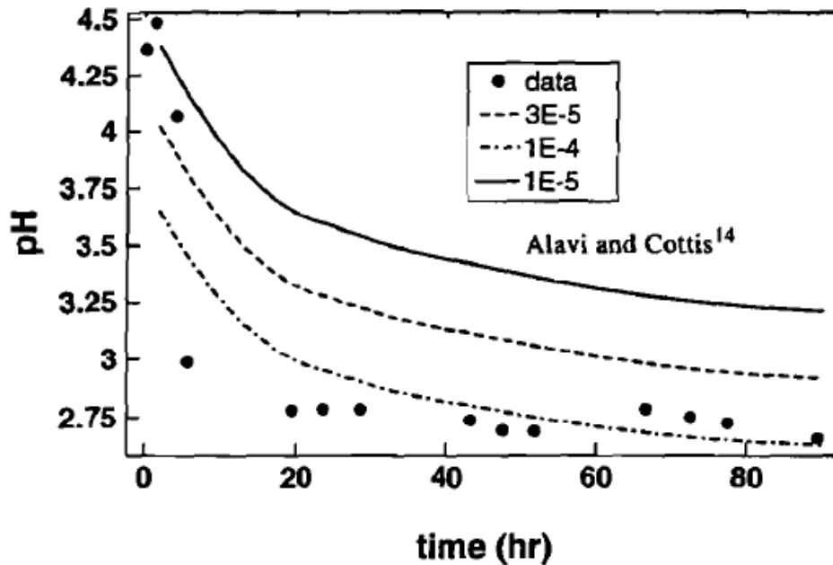
Figure 6. Experimental and Predicted pH values 7.5 cm into the Crevice as a Function of Time Using Different Constant Anodic Current Densities (A/dm 2 ) [Walton, et al. 20 , permission by Elsevier]
