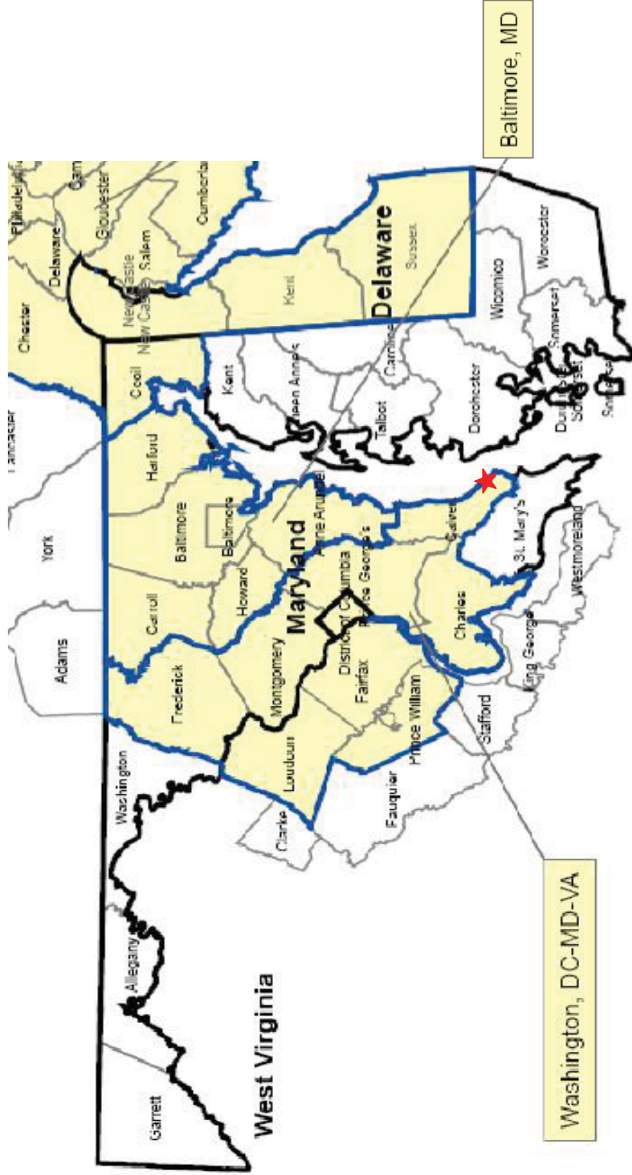
Figure 1-1 Washington, DC-MD-VA and Baltimore, MD 8-hr Ozone Nonattainment Regions
