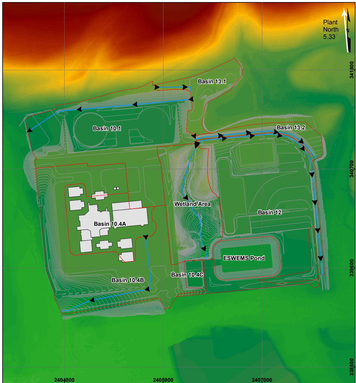
Figure 2.3-5— Site Drainage Flow Pattern
