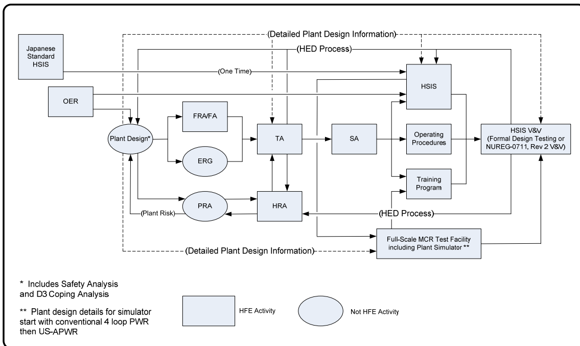
Figure 2.1-1 HFE Overall Work Flow, Reference MUAP-09019 R0, part 1
