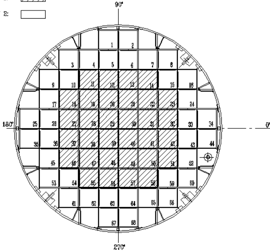
Figure 2.1-4 Fuel Loading Regions - MPC-68/68FF/68M
