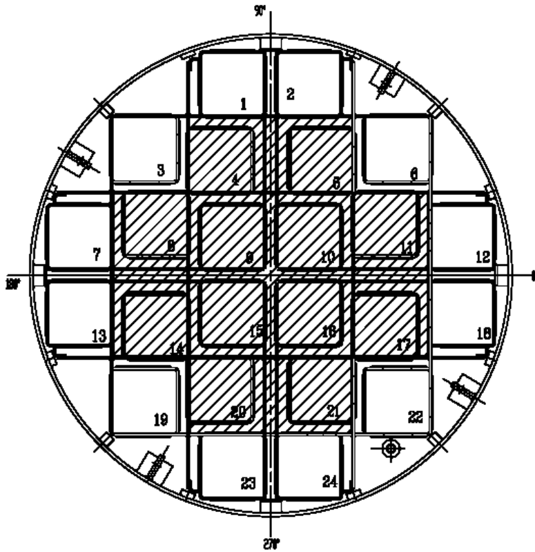
Figure 2.1-2 Fuel Loading Regions - MPC-24E/24EF
