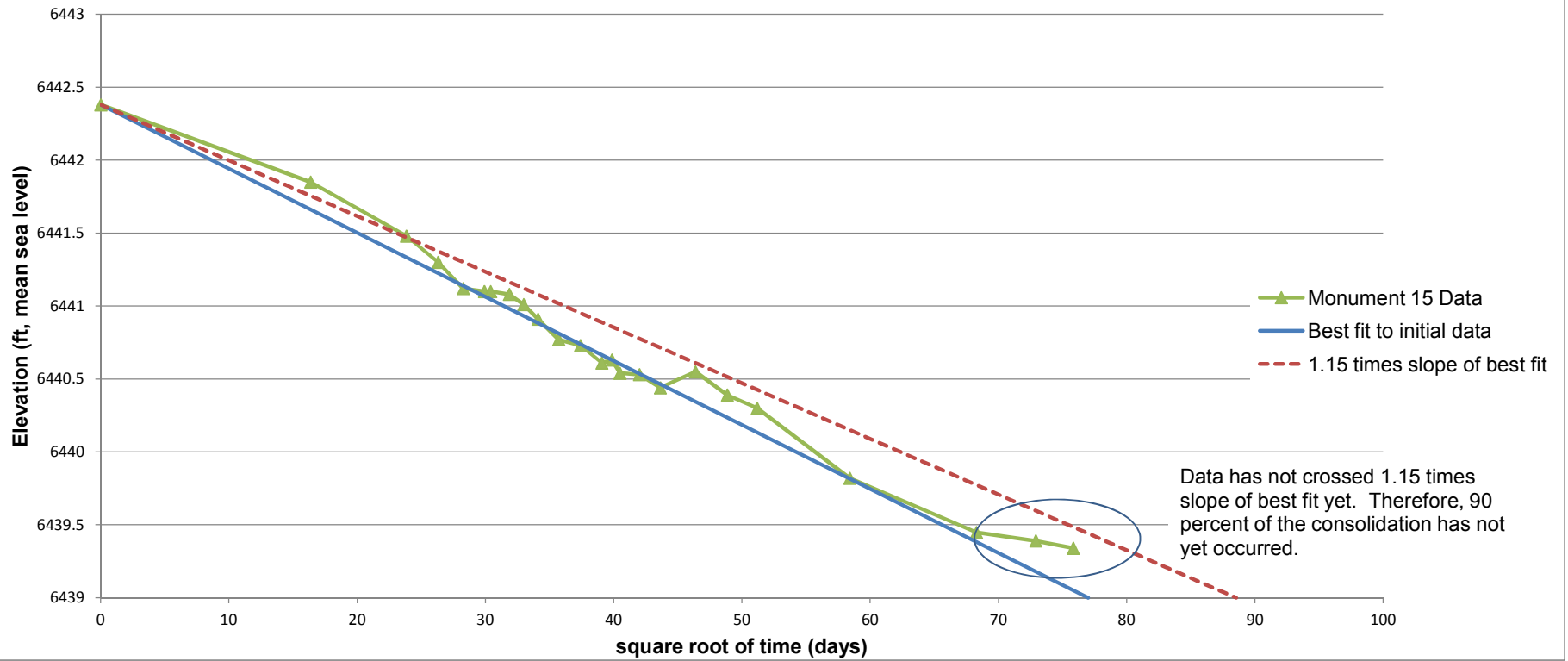
Figure 2 Settlement at Monument 15 (Old Monument DS2)
