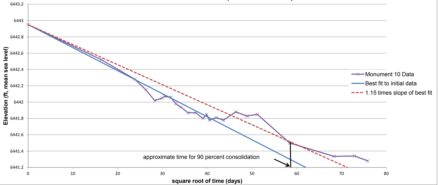
Figure 4 Settlement at Monument 10 (Old Monument DS4)
