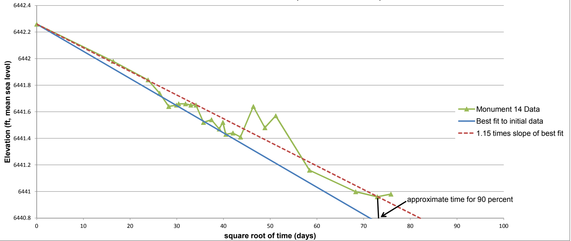
Figure 3 Settlement at Monument 14 (Old Monument DS3)
