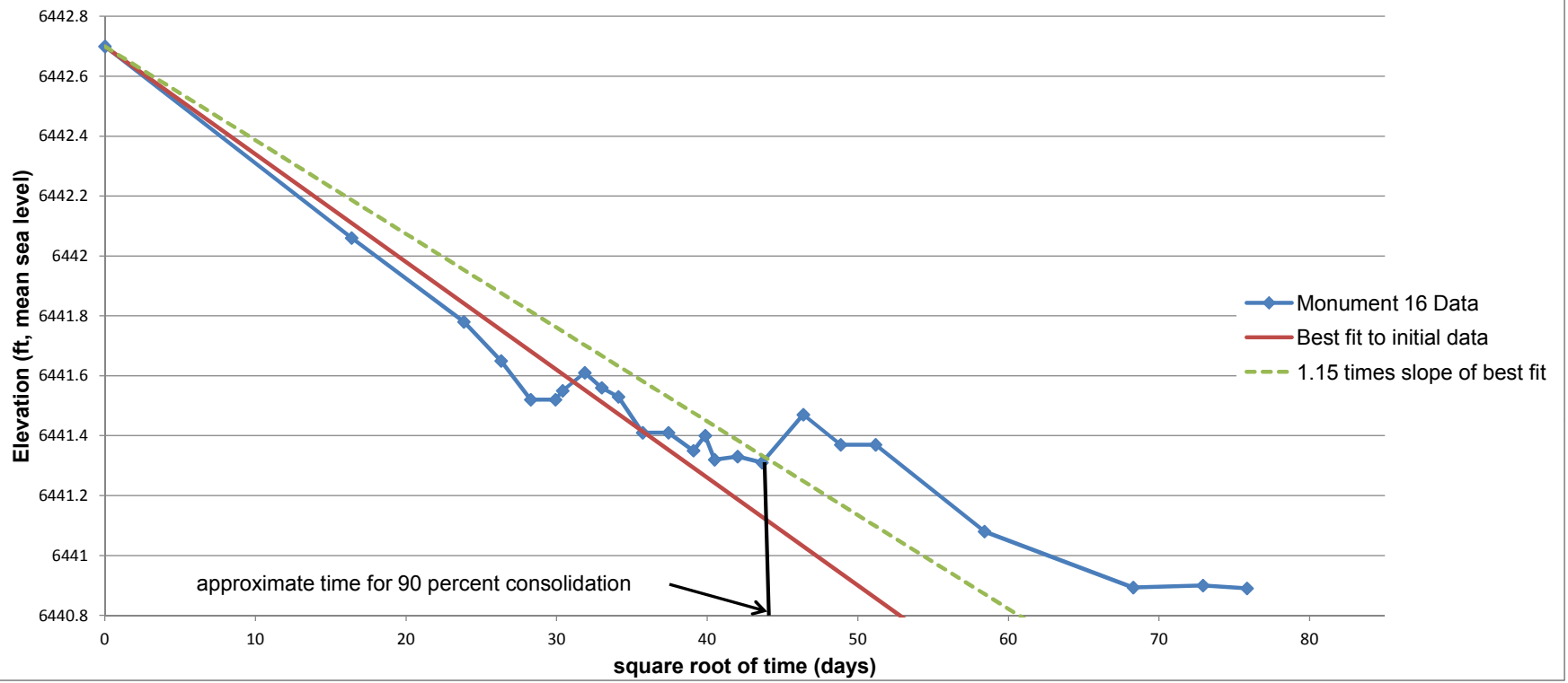
Figure 1 Settlement at Monument 16 (Old Monument DS1)
