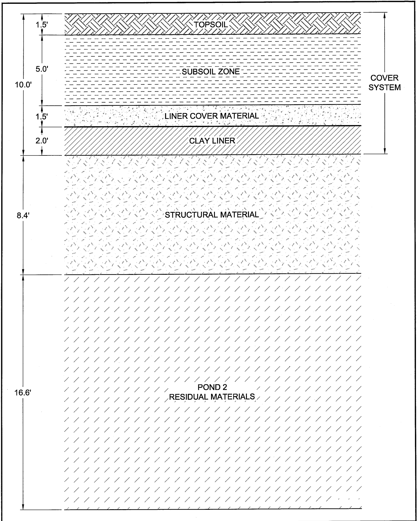
FIGURE C.4 PHASE IIB AREA TYPICAL INTERIOR CELL PROFILE
