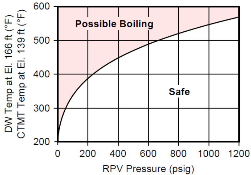
Fig 2: RPV Saturation Temperature (RPVST)
