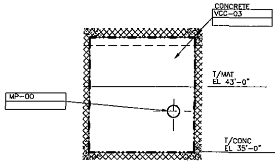
CONCRETE INSPECTION ZONE IWL-034-003 (EXTERIOR DEVELOPED VIEW, LOOKING FROM OUTSIDE)
