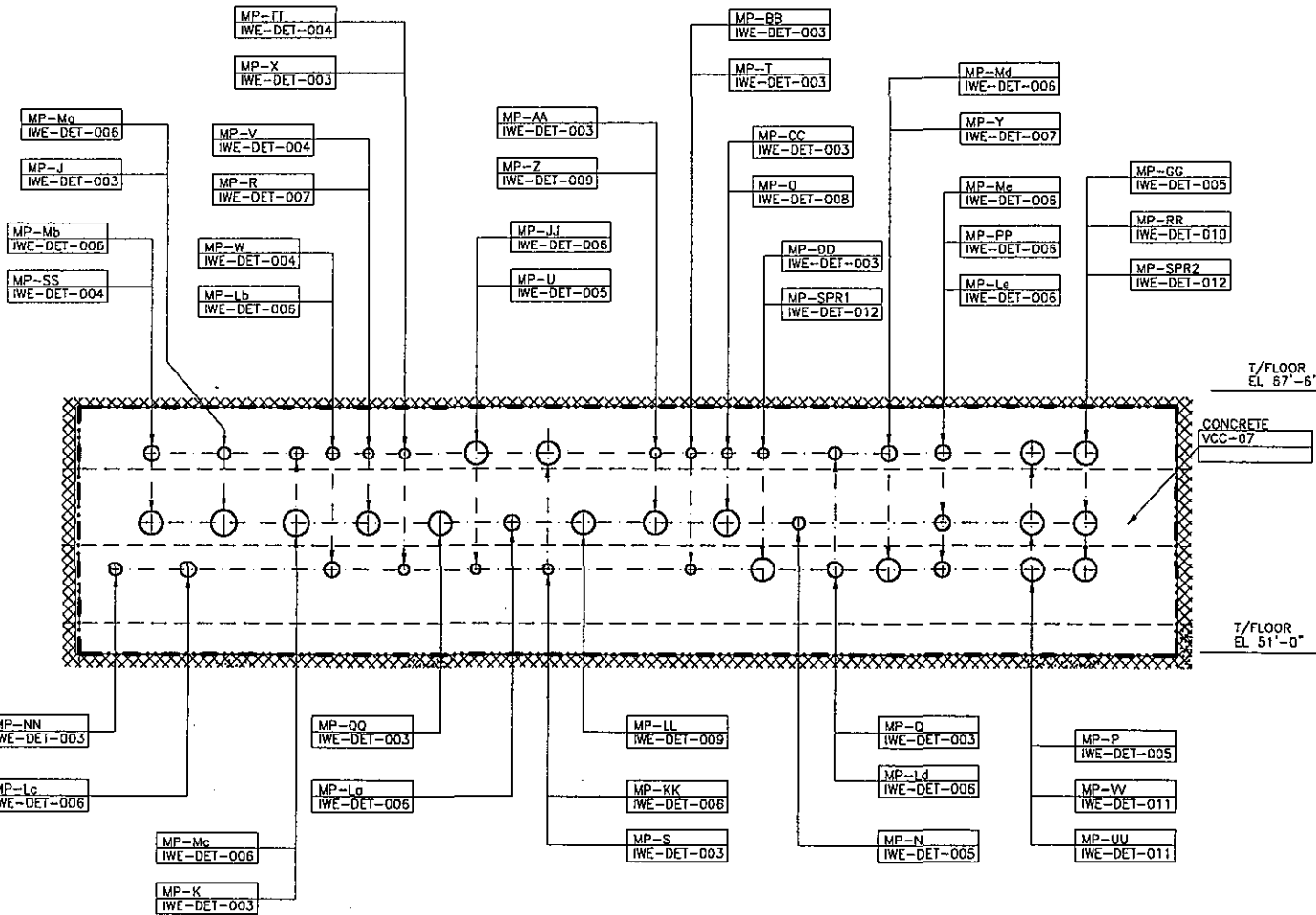
CONCRETE INSPECTION ZONE IWL-043-004 (EXTERIOR DEVELOPED VIEW, LOOKING FROM OUTSIDE)
