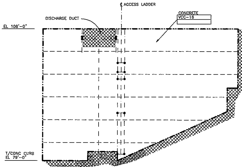
CONCRETE INSPECTION ZONE IWL-088-005 (EXTERIOR DEVELOPED VIEW, LOOKING FROM OUTSIDE)
