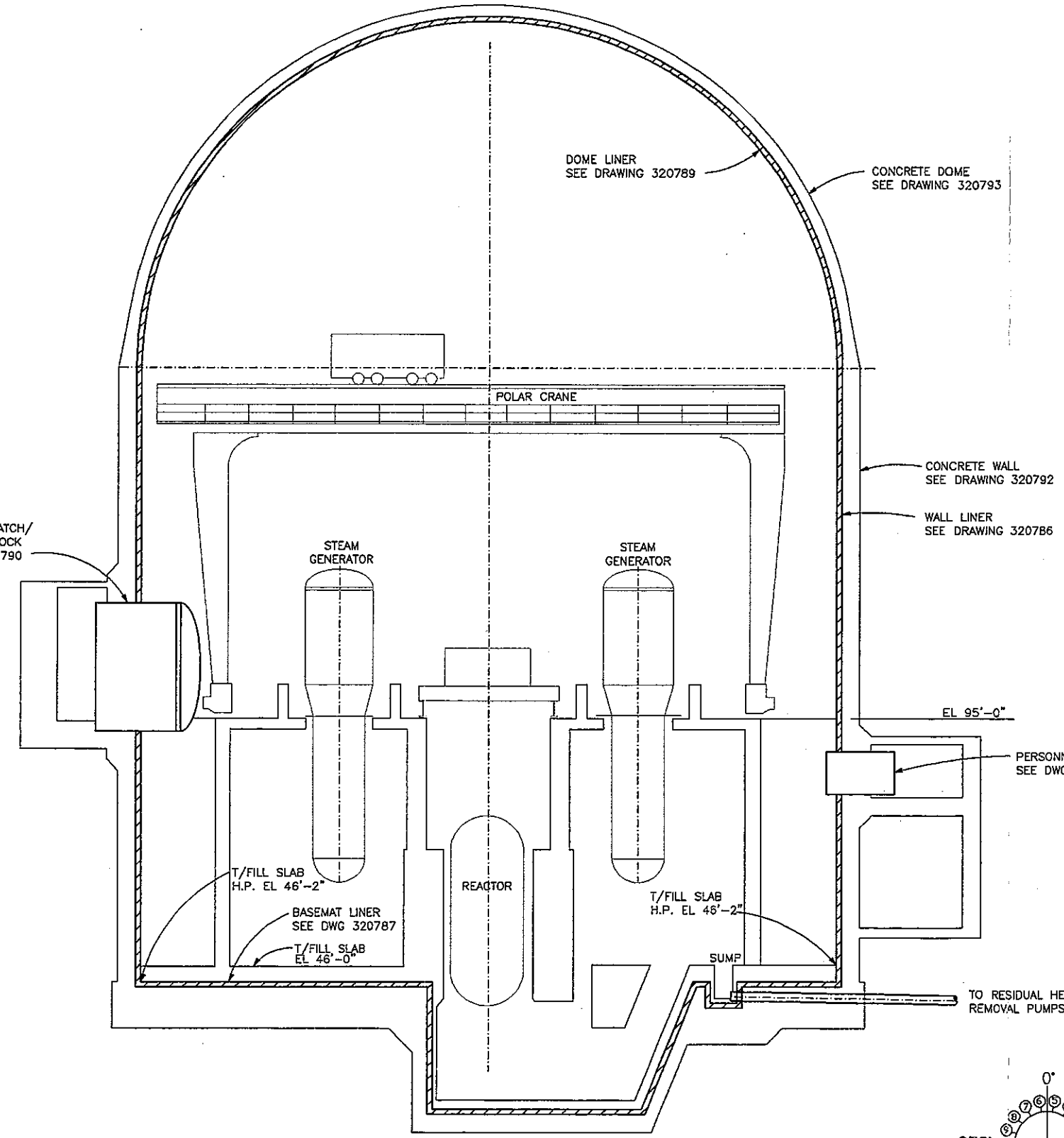
CONTAINMENT ISI GENERAL ARRANGEMENT
