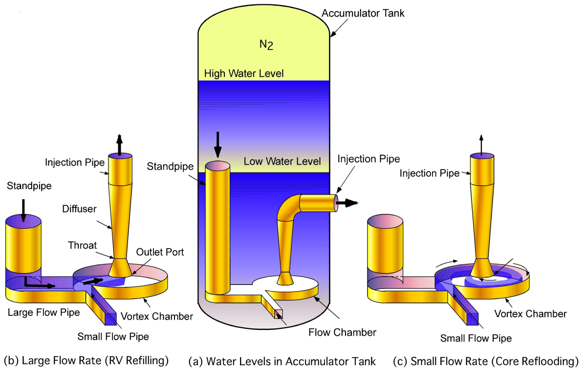
Figure 3.5-1 Principle of Advanced Accumulator
