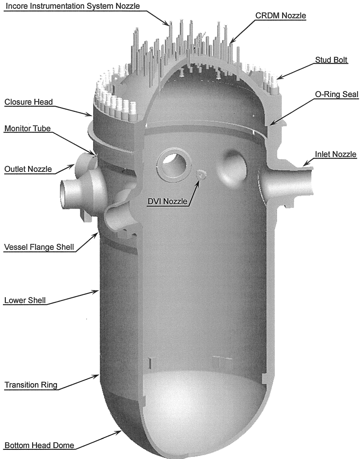
Figure 2-4 Reactor Vessel
