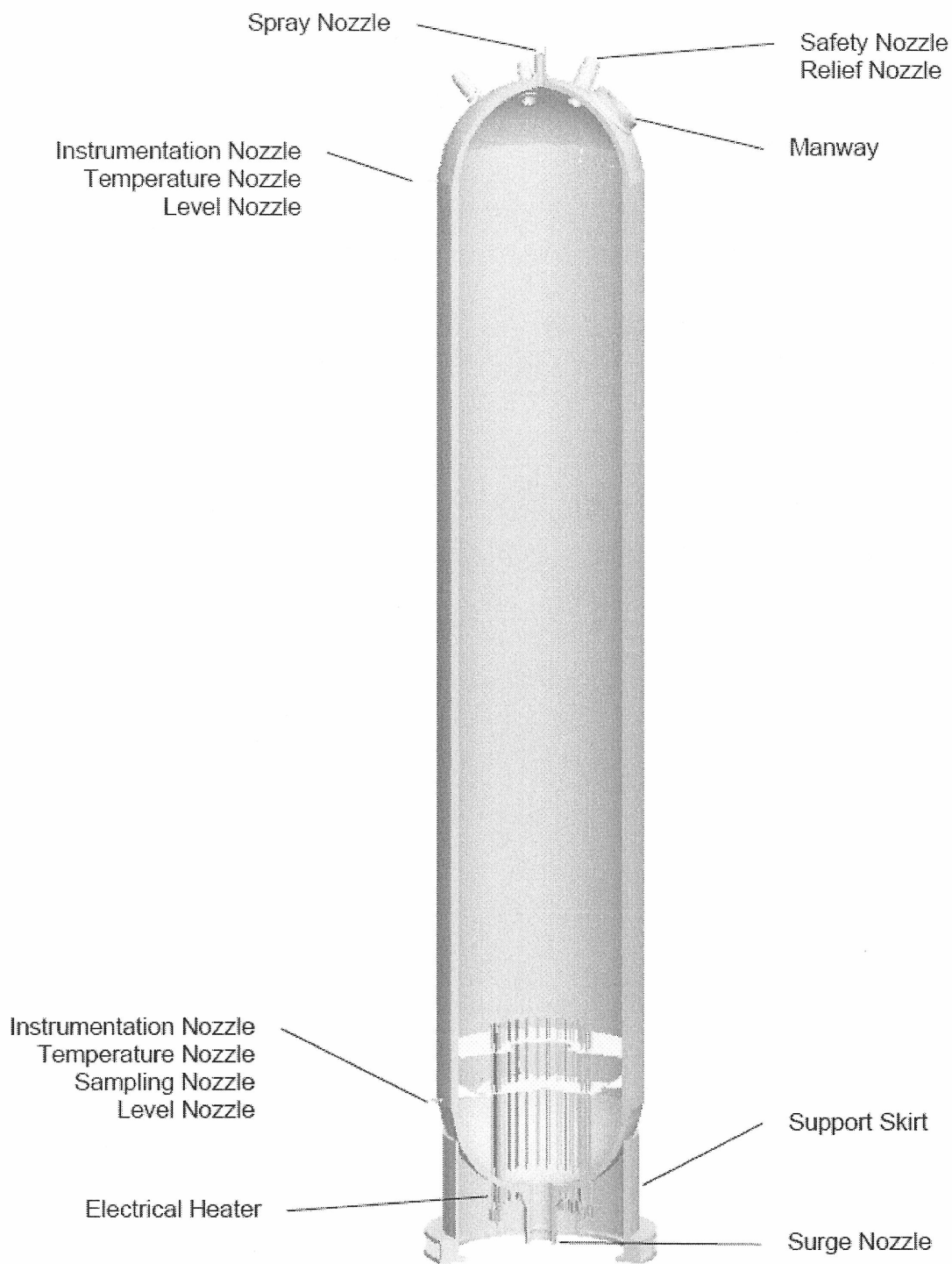
Figure 2-7 Pressurizer
