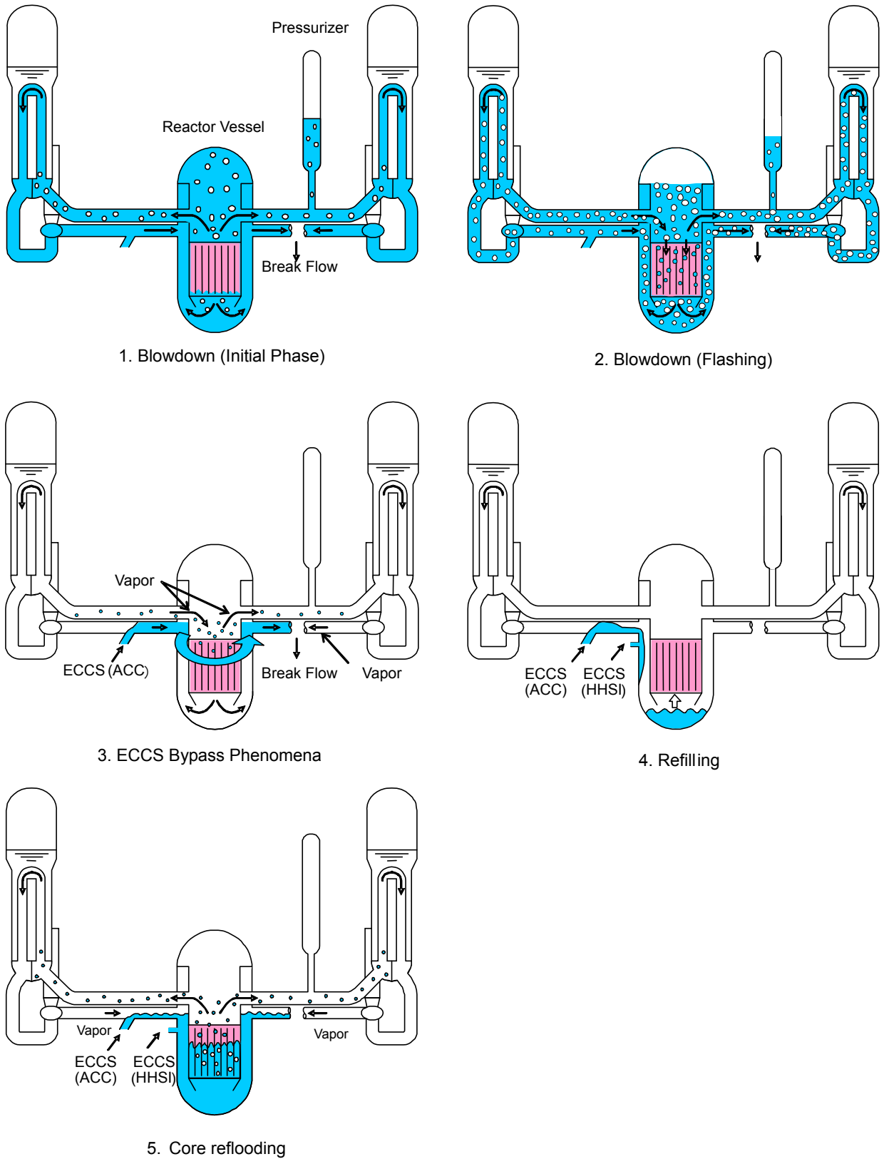
Figure 3.3-3 Transient of LBLOCA in US-APWR
