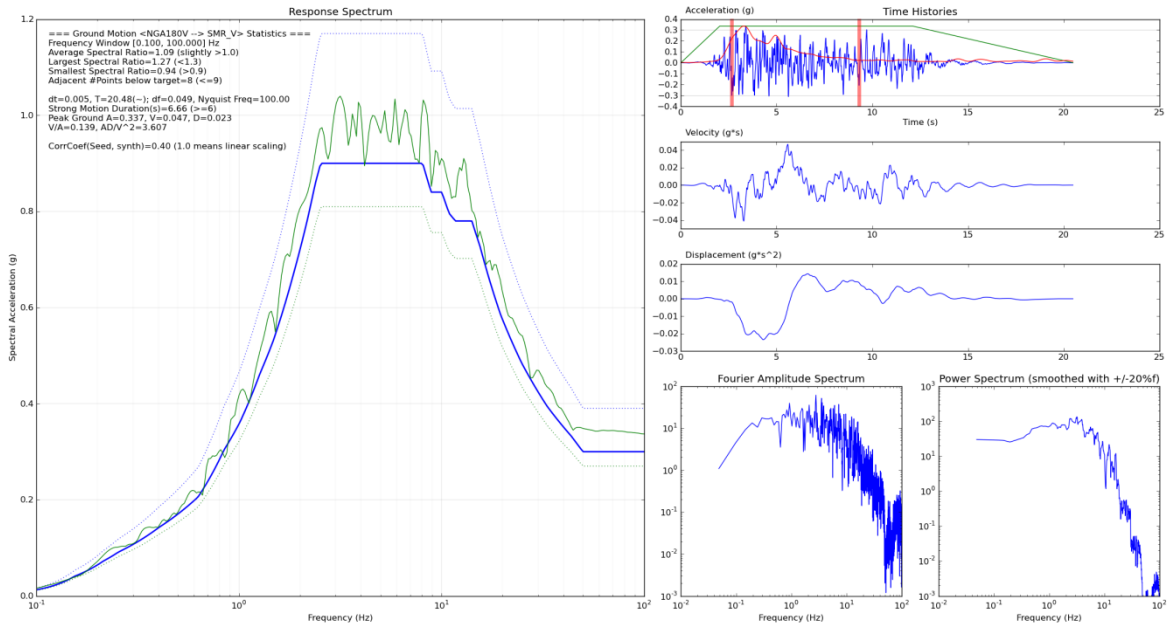
Figure 3-15 Synthetic Record SMR_V based on Seed Record NGA 180 V
