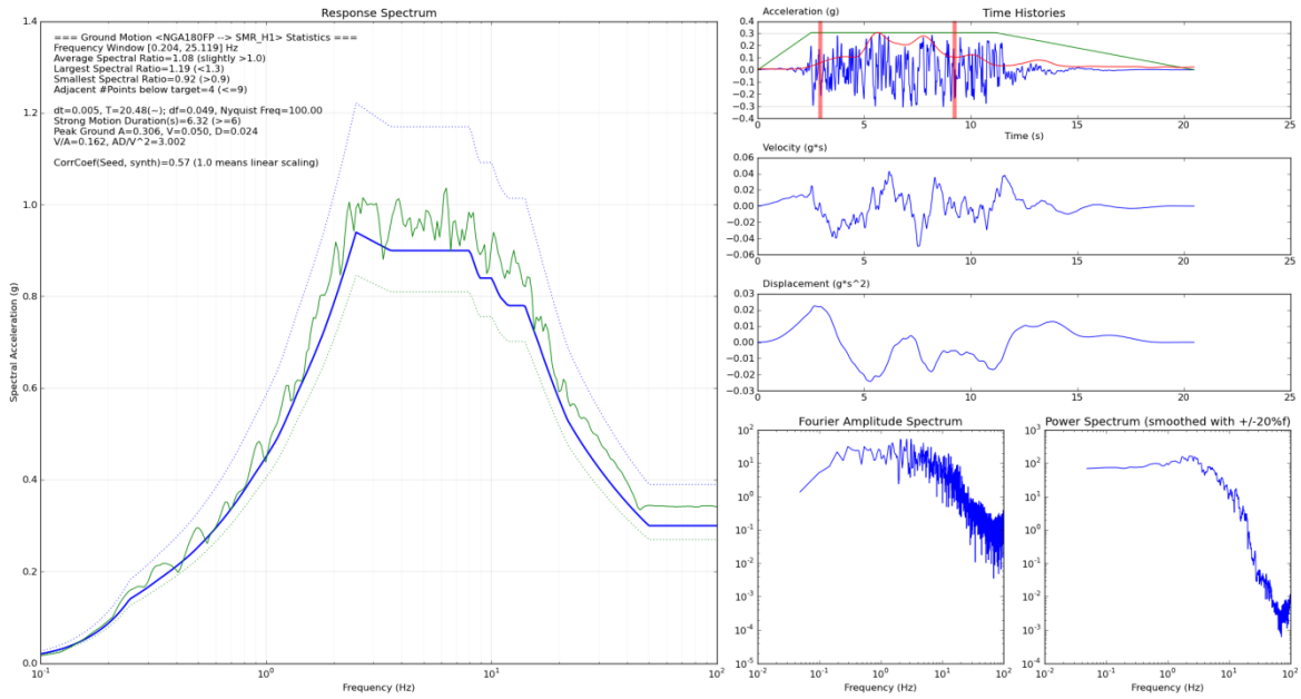
Figure 3-11 Synthetic Record SMR_H1 based on Seed Record NGA 180 FP
