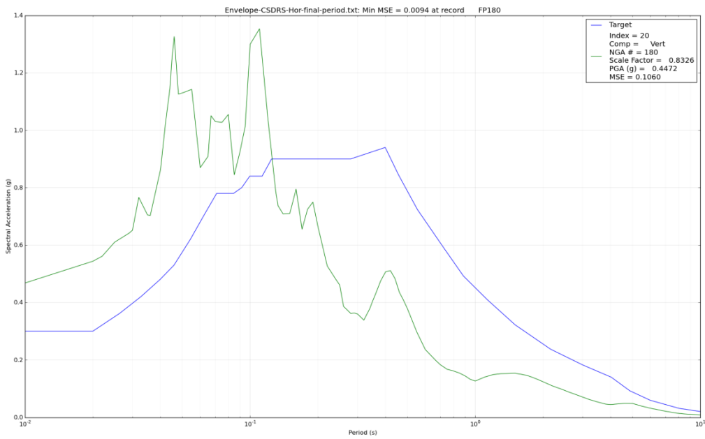
Figure 3-5 Comparison of NGA180 Vertical and Horizontal Envelop Spectrum
