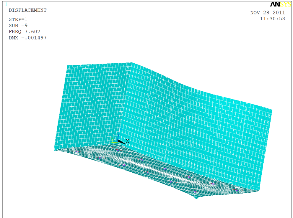
Figure 4-12 Mode Shape 9: Long Wall and Basemat
