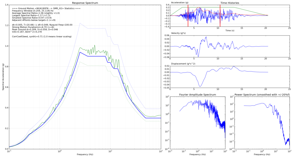
Figure 3-13 Synthetic Record SMR_H2 based on Seed Record NGA 180 FN
