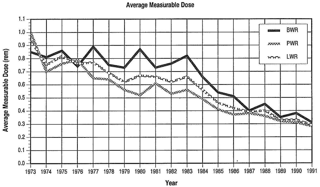
Figure 4.3 Average Measurable Dose and Collective Dose per Megawatt-Year 1973 – 1991
