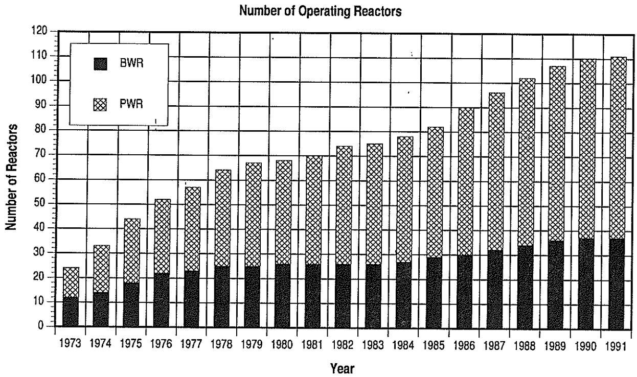
Figure 4.2 Number of Operating Reactors and Gross Electricity Generated 1973 – 1991
