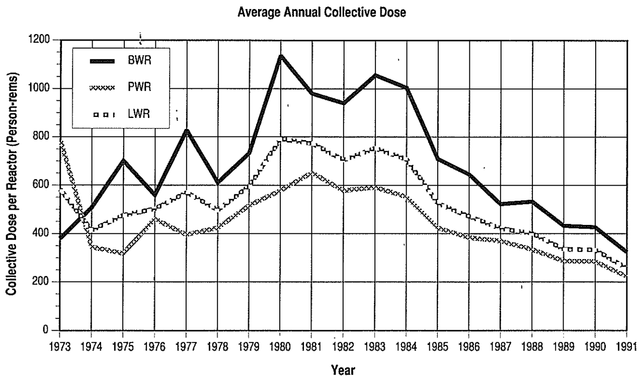
Figure 4.1 Average Collective Dose and Number of Workers per Reactor 1973 – 1991
