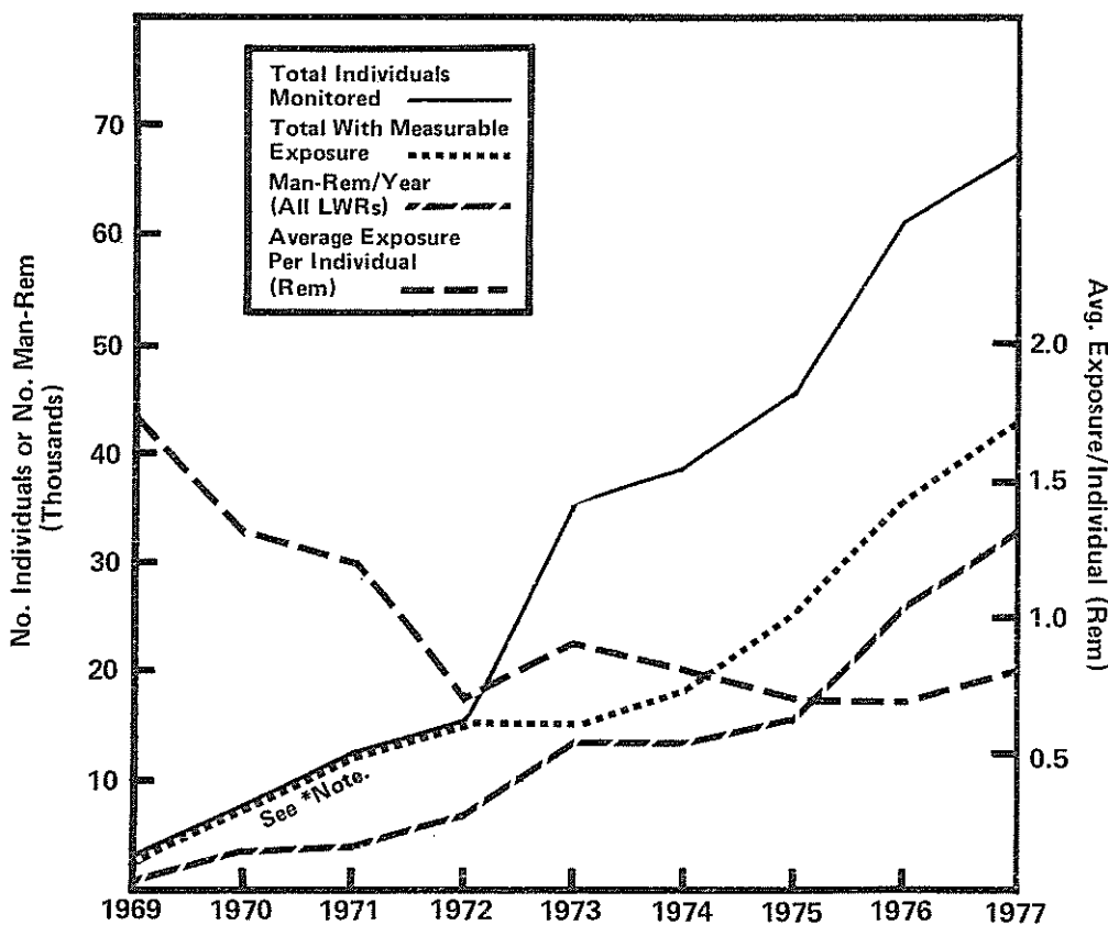
FIGURE 3 AVERAGE EXPOSURE PER INDIVIDUAL 1969-1977
