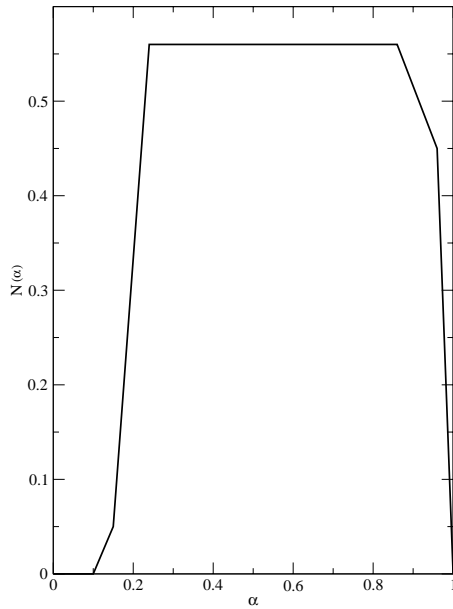
Figure. 2-55. Semiscale torque degradation multiplier curve.
