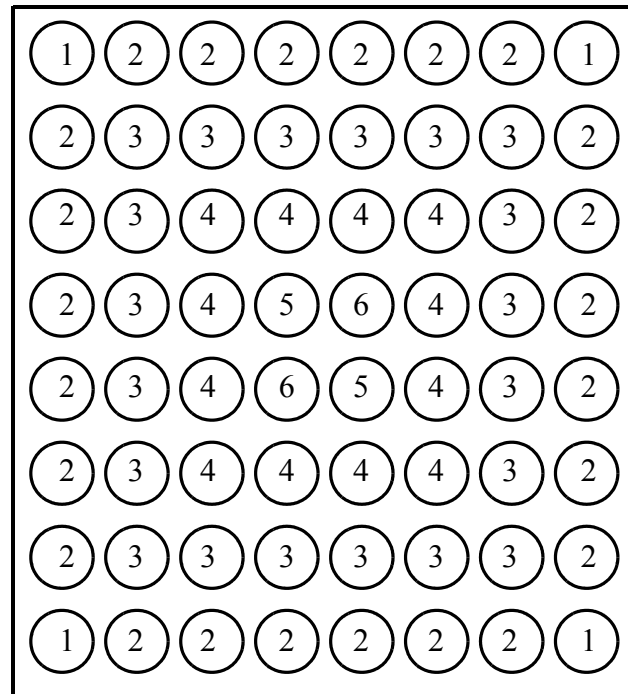
Figure. 2-31. 8x8 Fuel Assembly Simulated with 6 Rod Groups.
