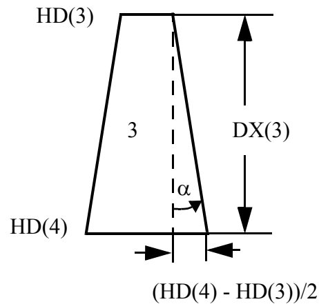
Figure. 2-41. Diffuser Angle.
