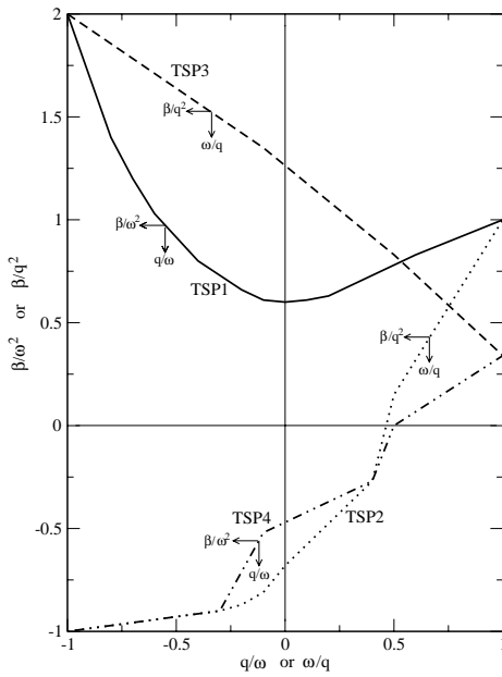
Figure. 2-59. LOFT single-phase homologous torque curves.
