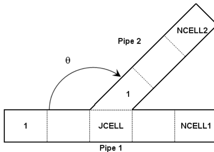
Figure. 2-73. TEE-component noding diagram.
