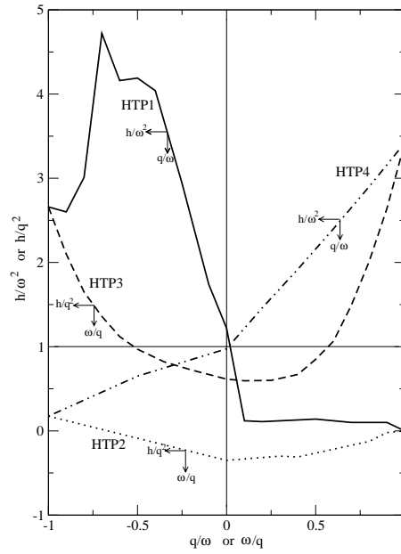
Figure. 2-52. Semiscale two-phase fully degraded homologous pump-head curves.
