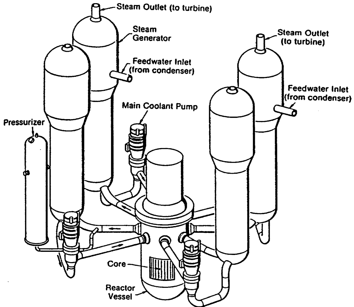
Figure. 3-1. PWR Primary Coolant System.
