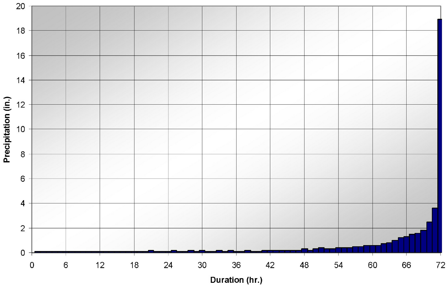
WILLIAM STATES LEE III NUCLEAR STATION UNITS 1 & 2 Local Intense Probable Maximum Precipitation 72-Hour End Peaking Hyetograph FIGURE 2.4.3-236 Rev 2
