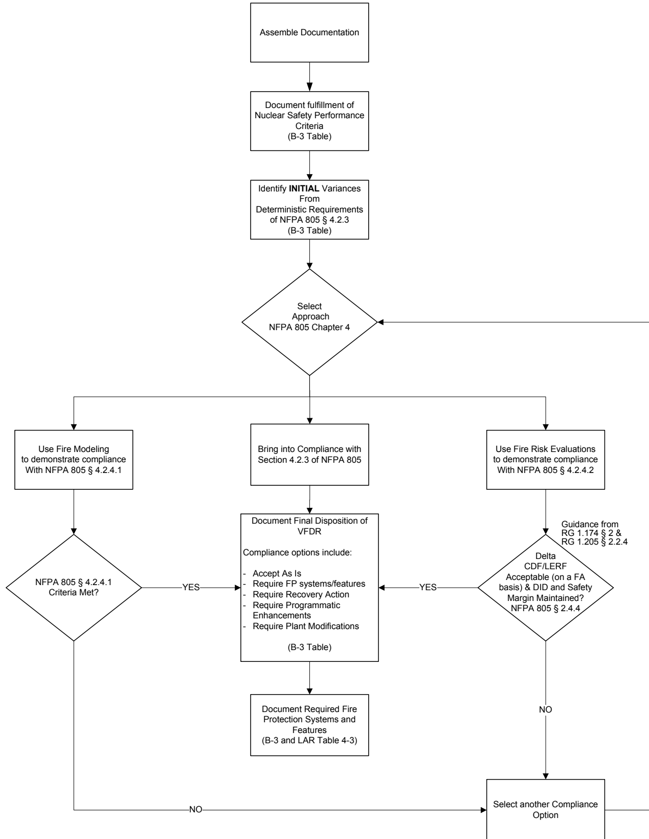
Figure B-TBD1 – NFPA 805 Chapter 4 Compliance Assessment Process
