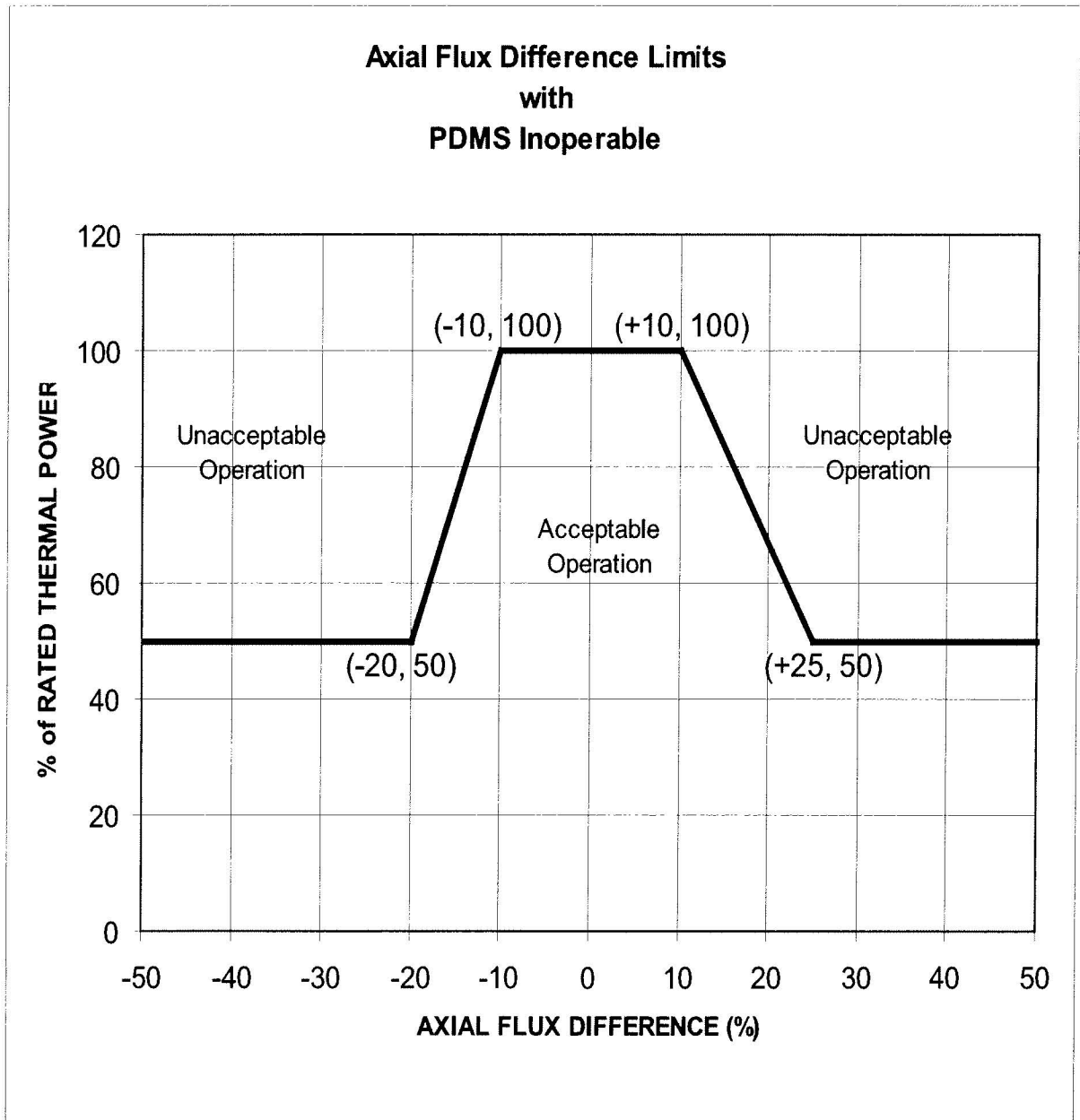
Figure 2.8.1.b: Reduced Axial Flux Difference Limits as a Function of Rated Thermal Power (Cycle burnup \geq 18000 MWD/MTU)
