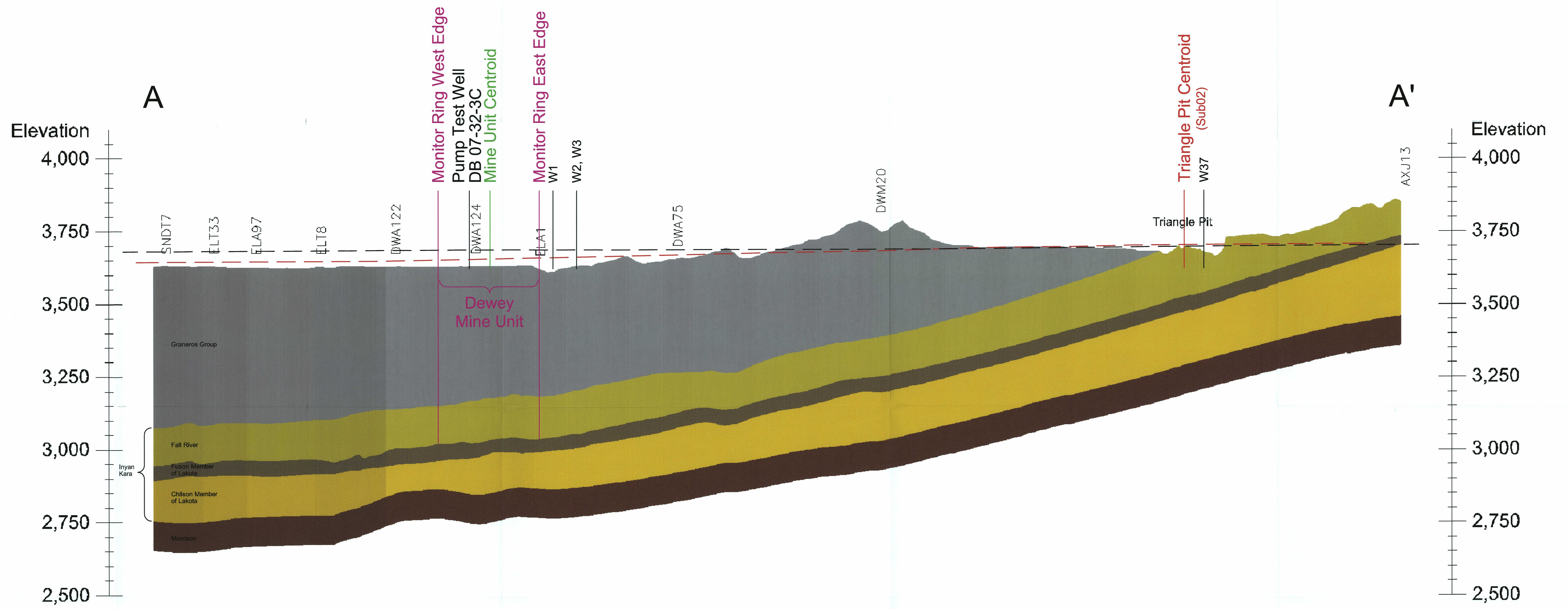
Dewey-Burdock (North) Cross Section
