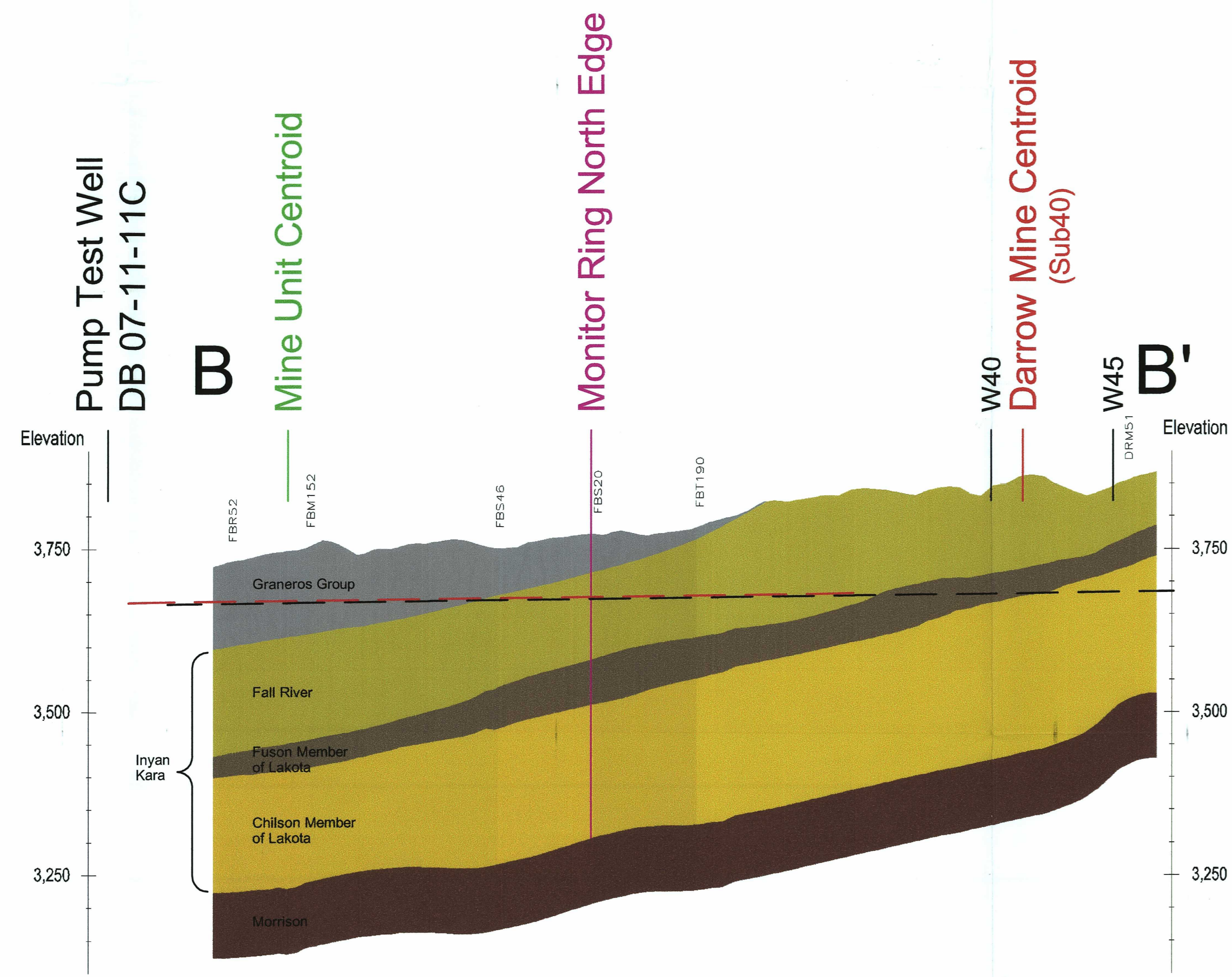
Burdock (South) Cross Section
