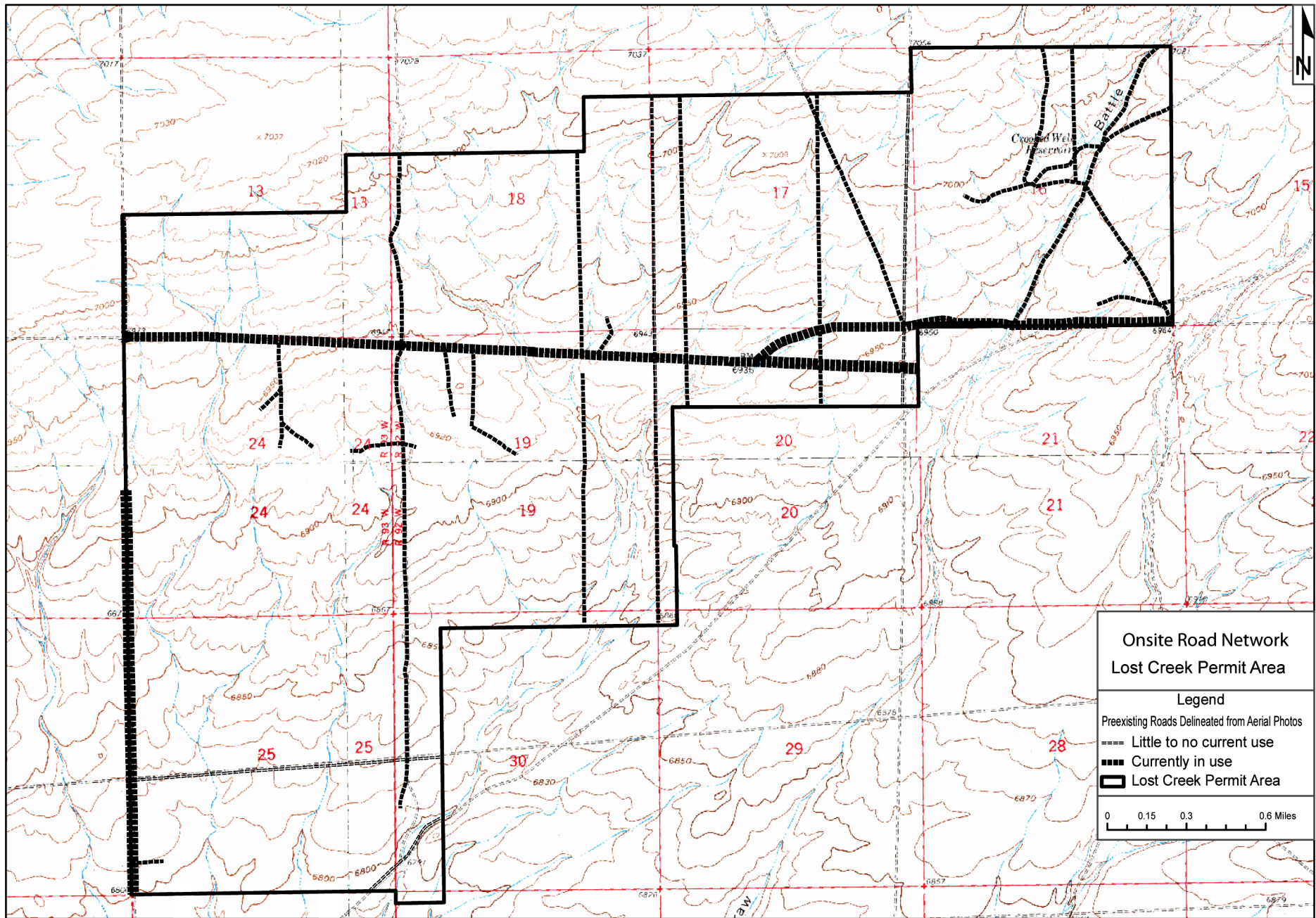
Figure 3-3 On-site Roads
