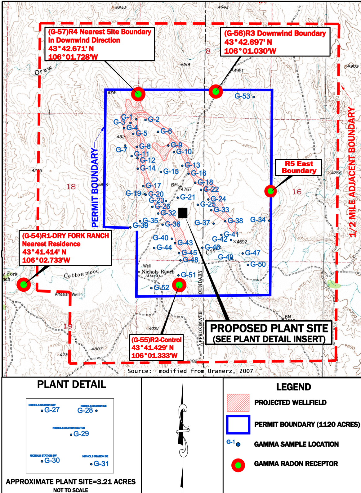
Figure 6-3. Nichols Ranch Unit Radon, Gamma, and Air Particulate Monitoring Locations
