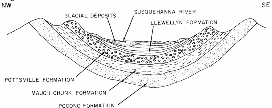
Figure 5. Generalized section through the Wyoming Valley synclinalorium showing the relations of Mississippian and younger age rocks.
