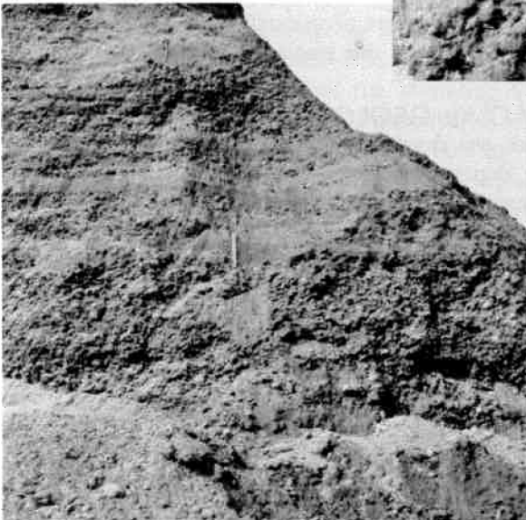
Figure 8. Photographs showing glacial outwash sediments, 1 mile west of Wyoming.
