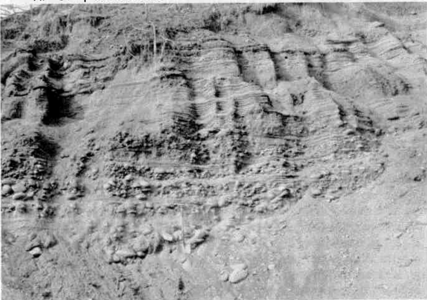
B. Simple structure; 0.25 miles northwest of Duryea.
