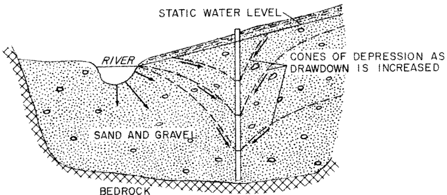
Figure 11. Illustration of the cone of depression developed when a well is pumped where recharge is induced from a perennial stream.
