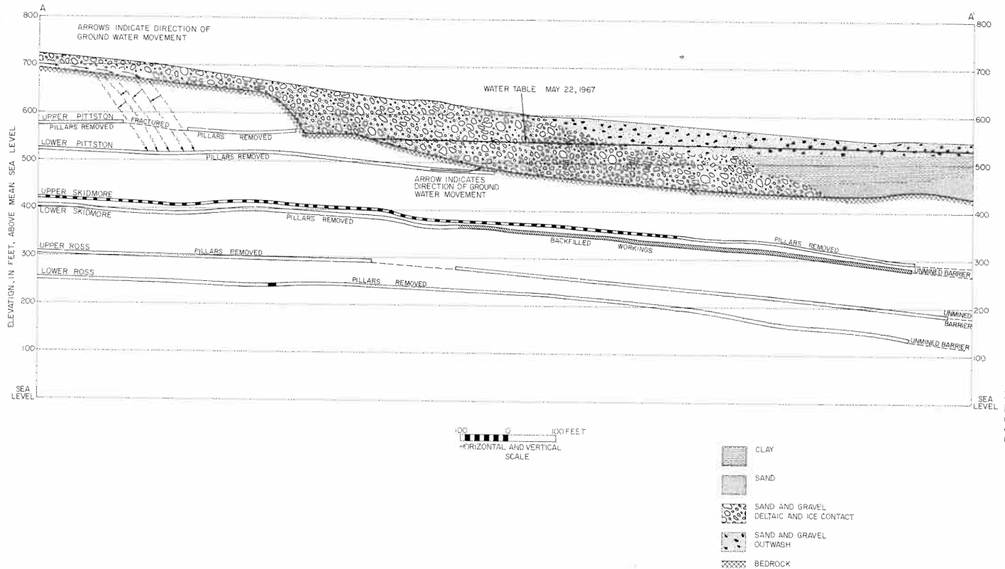
Figure 12. Section through the Harry E. mine showing mined beds and relation to the buried valley.
