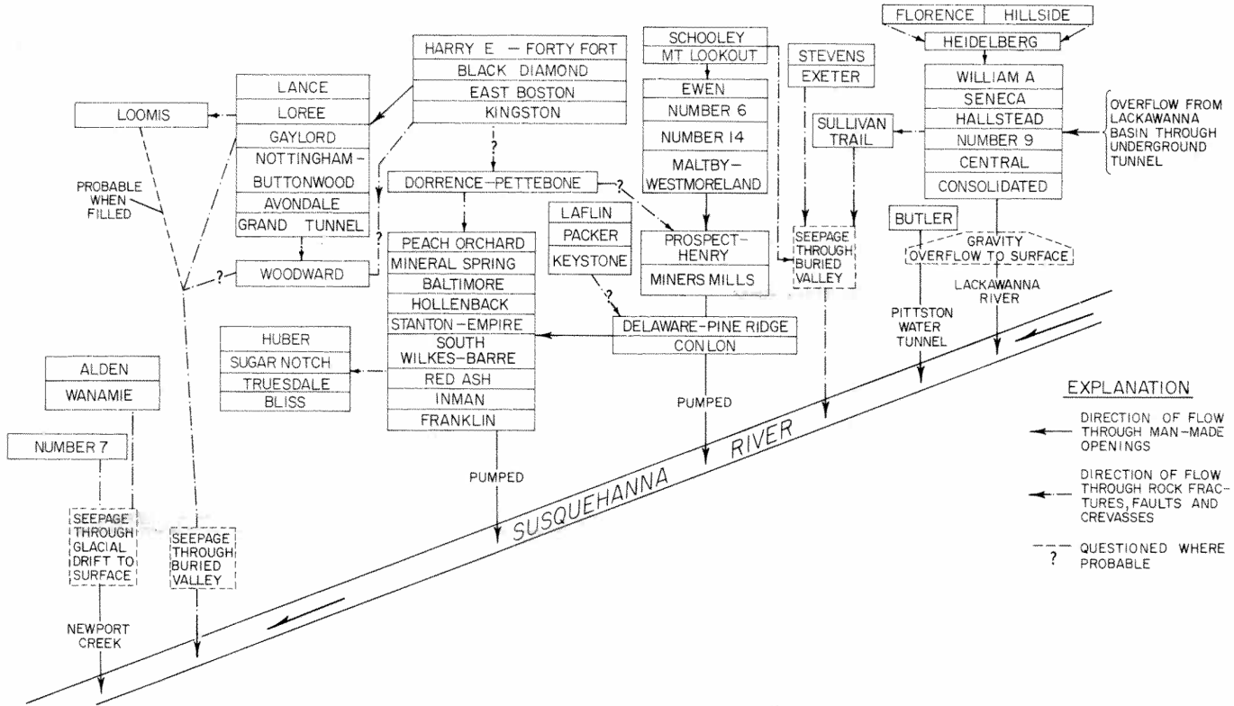
Figure 15. Schematic of water flow through the mines in the Wyoming Valley.
