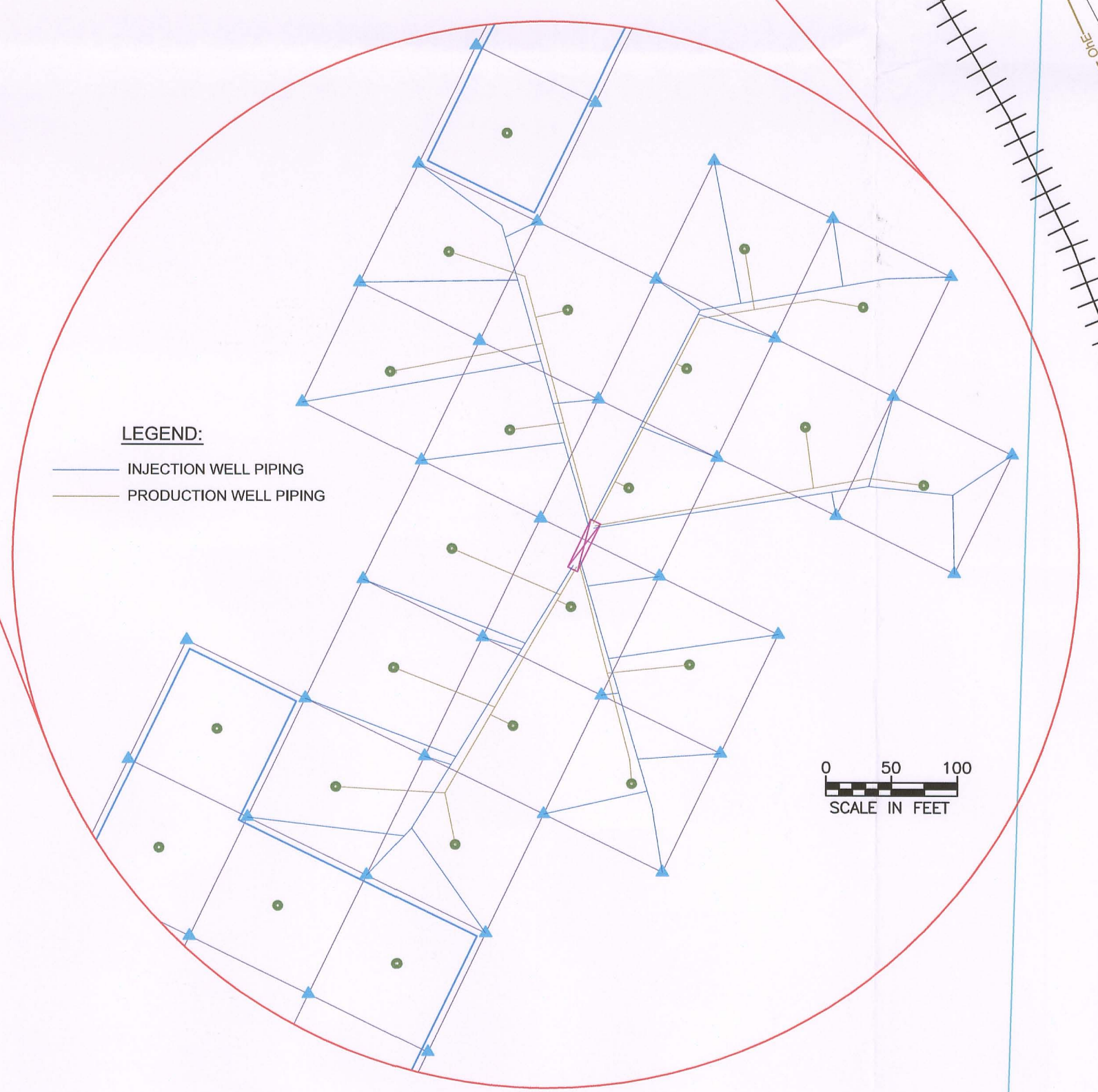
SIMPLIFIED HEADER HOUSE MINING UNIT PIPING LAYOUT
