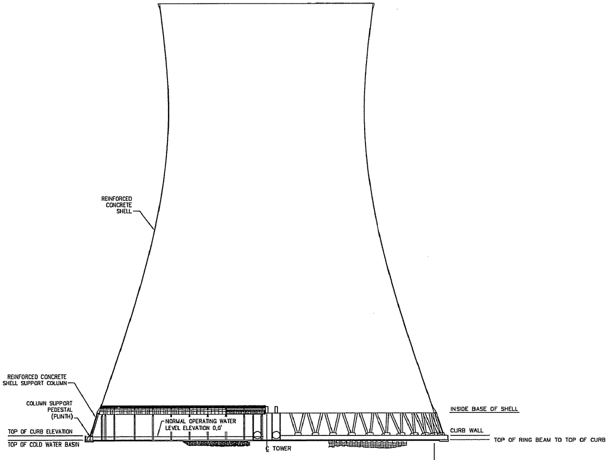
ELEVATION OF TOWER (A)
