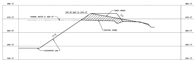
SECTION 3 (SIMILAR) TYPICAL SECTION EMBANKMENT ABOVE WATER LEVEL TO EL. 674'-0" SEE DWG 51101
