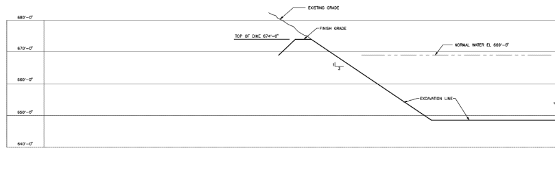
SECTION 2 (SIMILAR) TYPICAL CROSS-SECTION NO EMBANKMENT SEE DWG 51101
