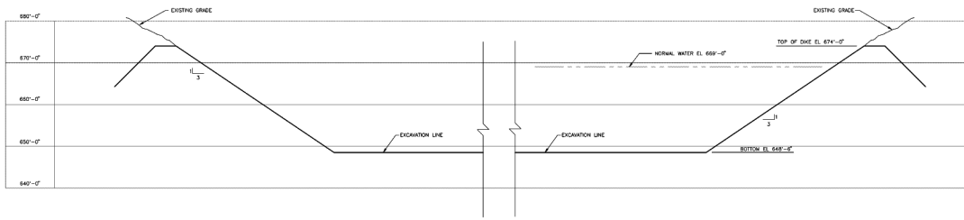
SECTION 1 (SIMILAR) SECTION AT EMBANKMENT SEE DWG 51101
