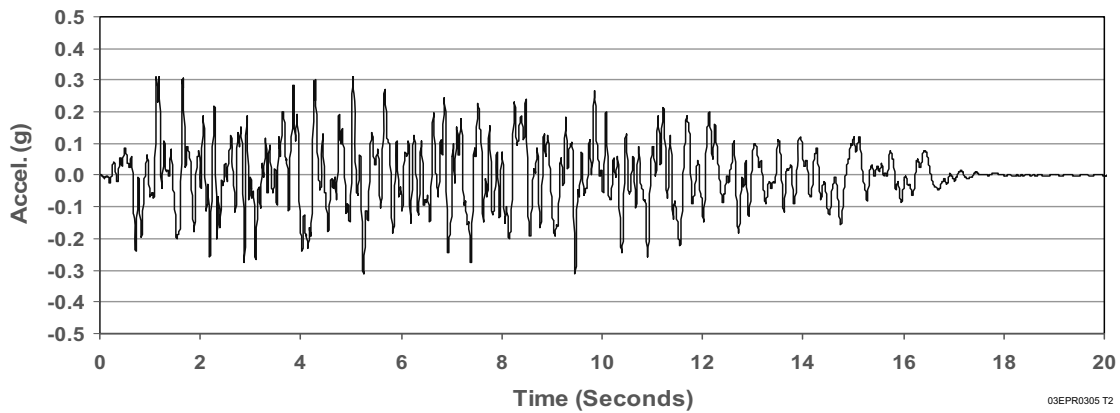
EURS3 - ACCELERATION TIME HISTORY
