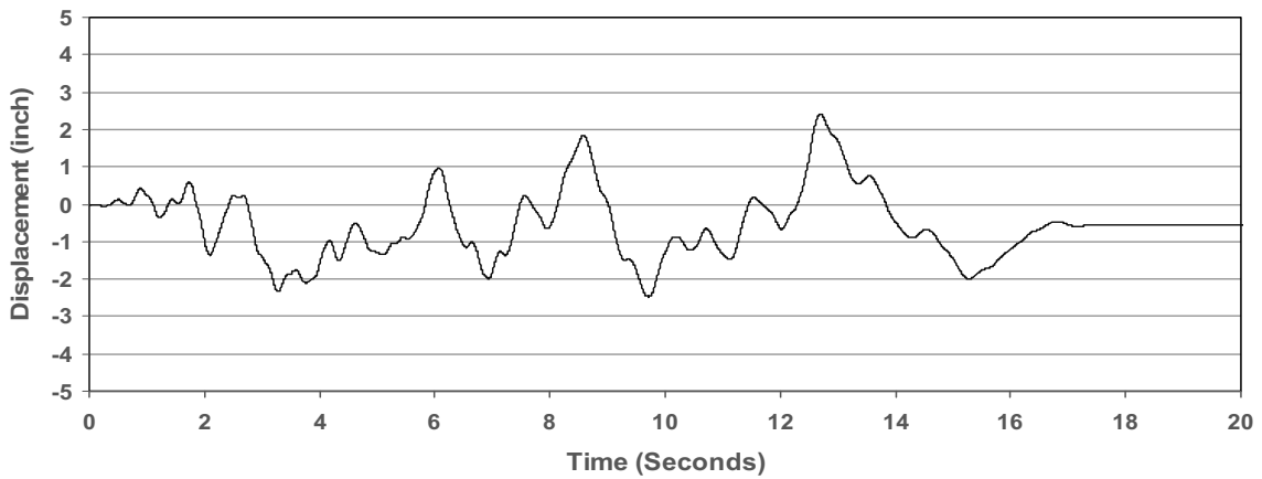
EURS3 - INTEGRATED DISPLACEMENT TIME HISTORY
