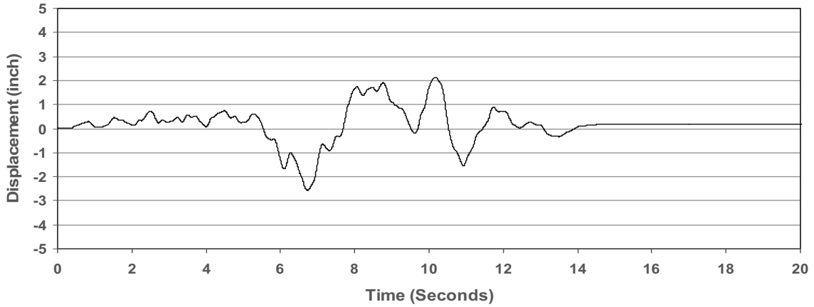
EURS2 - INTEGRATED DISPLACEMENT TIME HISTORY
