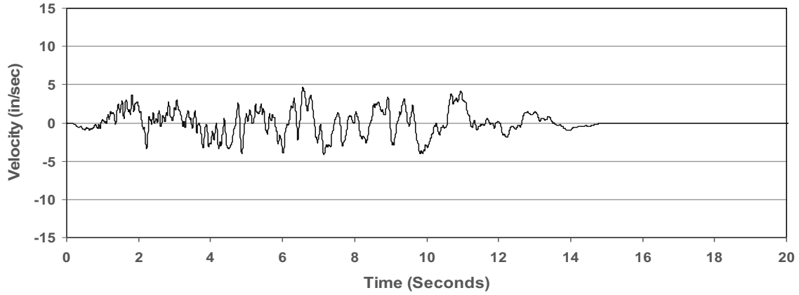
EURH2 - INTEGRATED VELOCITY TIME HISTORY
