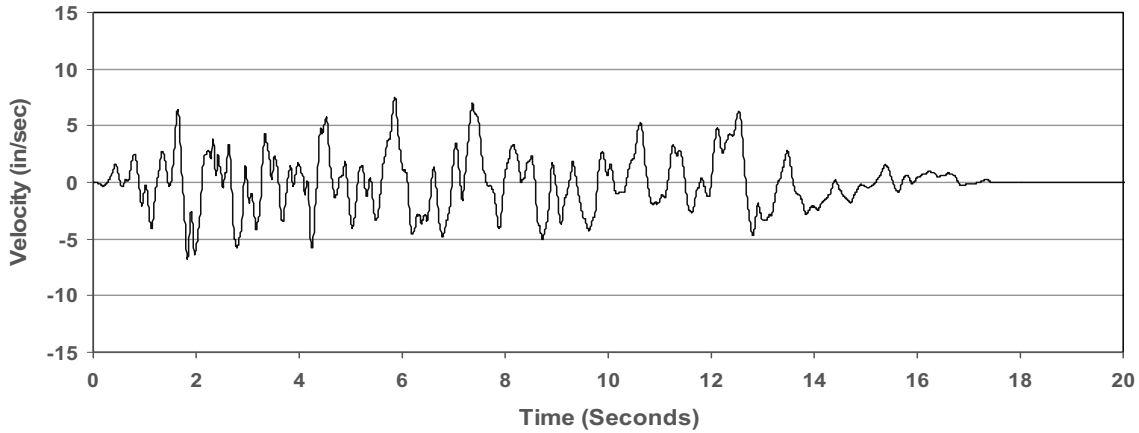
EURM2 - INTEGRATED VELOCITY TIME HISTORY
