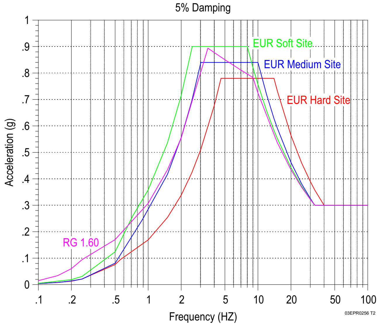
Figure 3.7.1-3—Comparison of CSDRS to RG 1.60, Vertical Motion
