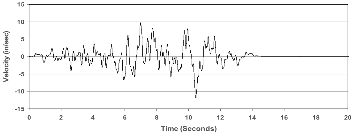
EURS2 - INTEGRATED VELOCITY TIME HISTORY
