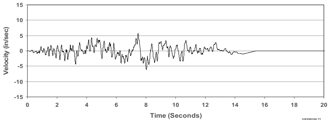
EURH3 - INTEGRATED VELOCITY TIME HISTORY
