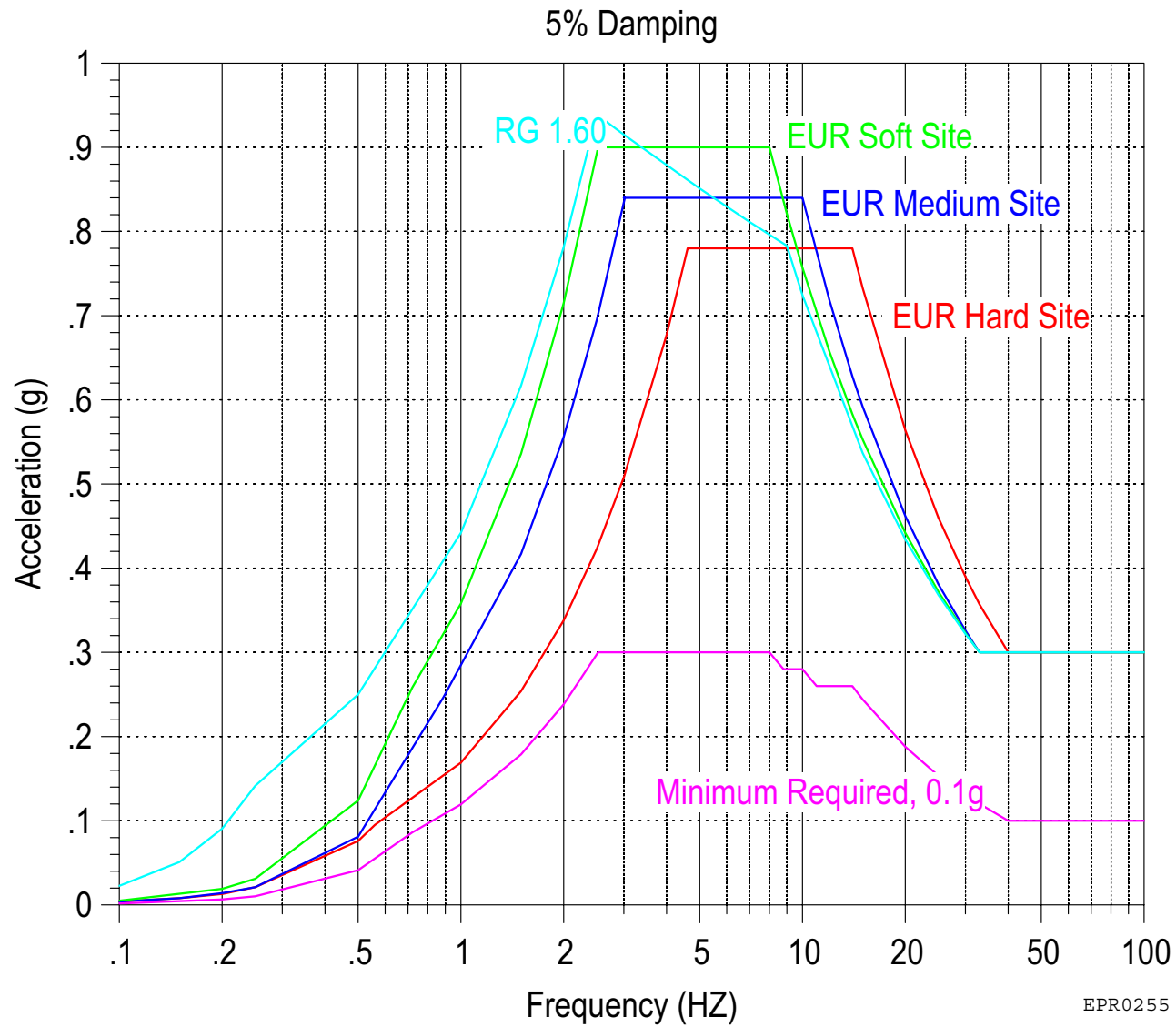
Figure 3.7.1-2—Comparison of CSDRS to RG 1.60 and the Minimum Required Spectrum, Horizontal Motion
