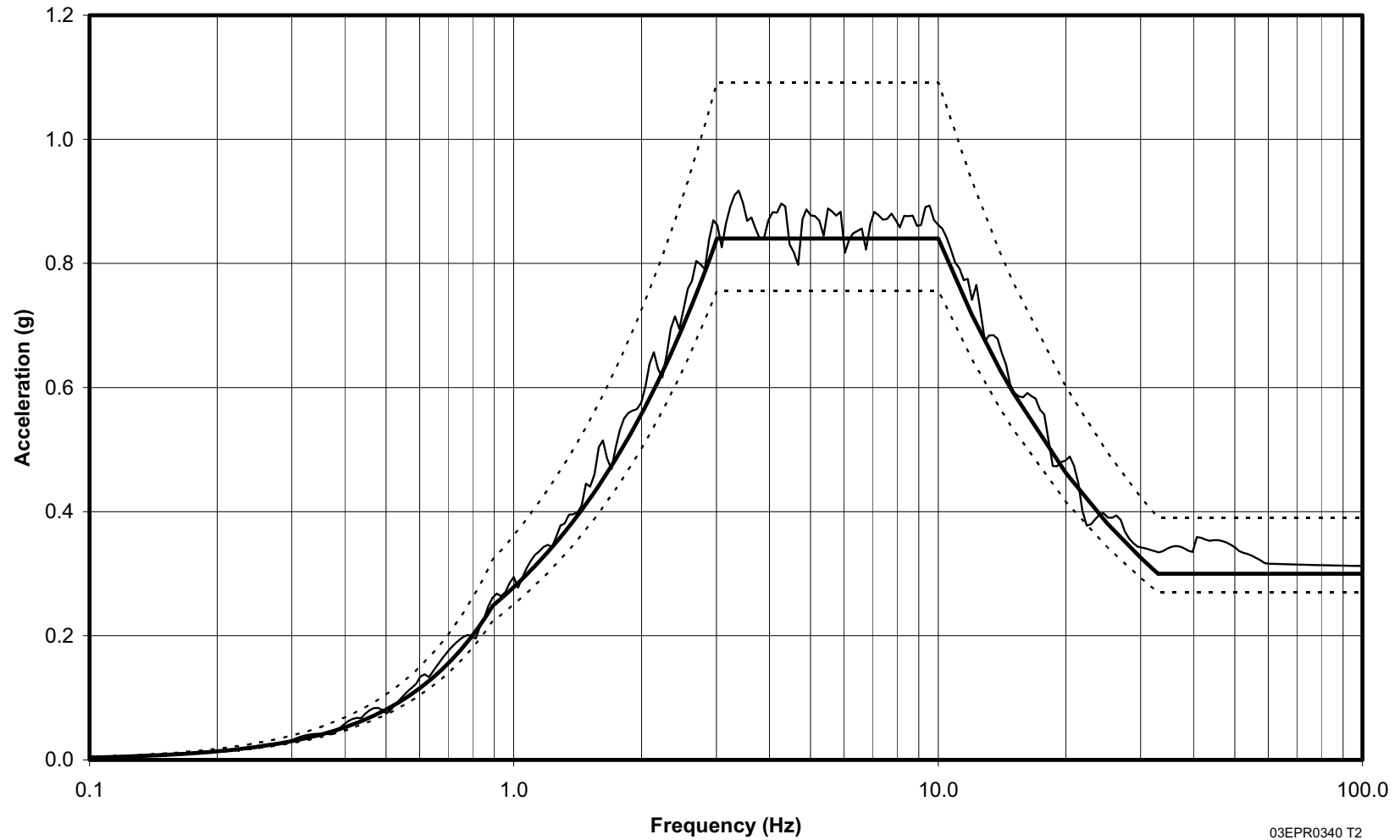
Figure 3.7.1-20—Response Spectrum of Time History H1 vs. Target Spectrum for EUR Hard Motion (TH1 Target, 1.30*Target and 0.90*Target at 5% Damping)
