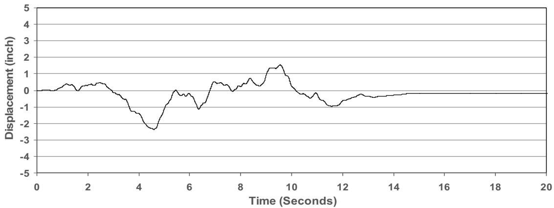
EURH3 - INTEGRATED DISPLACEMENT TIME HISTORY
