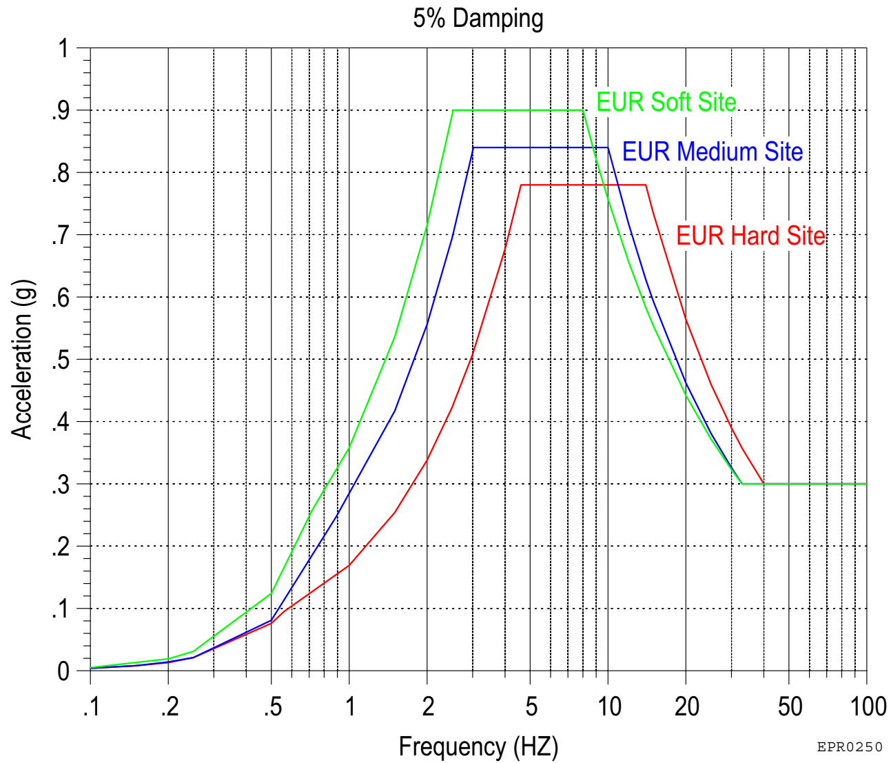
Figure 3.7.1-1—Design Response Spectra for EUR Control Motions (hard, medium and soft sites)
