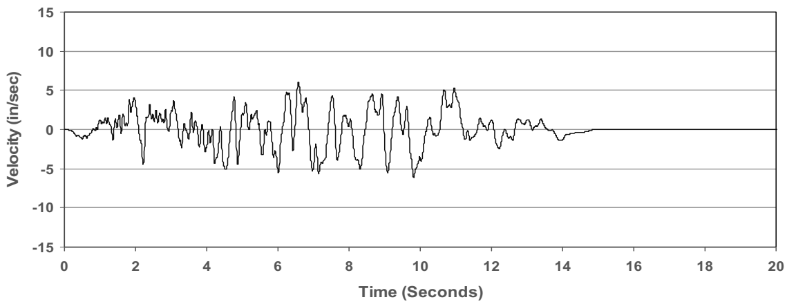
EURM3 - INTEGRATED VELOCITY TIME HISTORY
