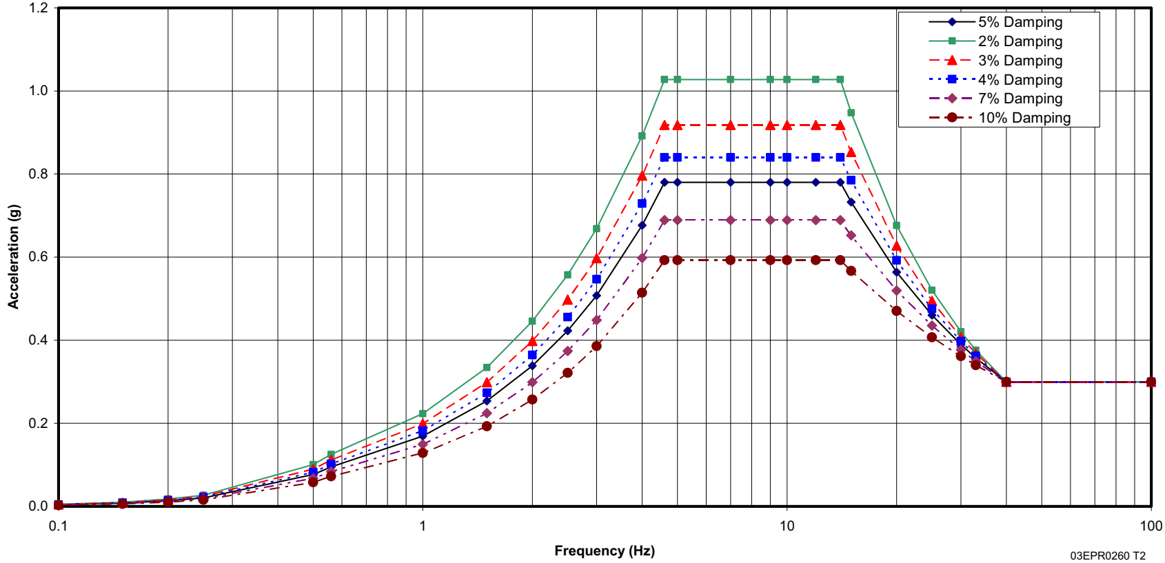
EUR Hard Design Ground Spectra, 0.3g
