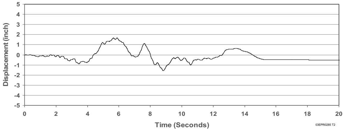
EURH3 - INTEGRATED DISPLACEMENT TIME HISTORY
