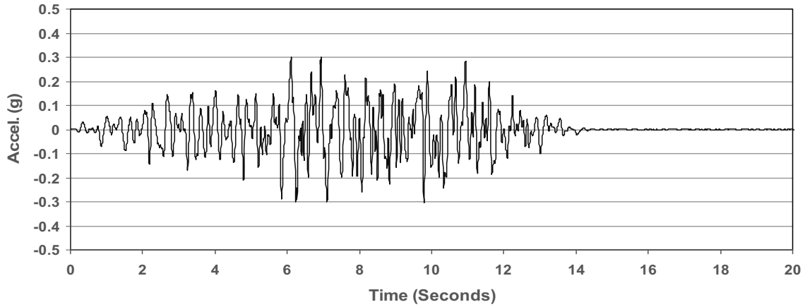
EURS2 - ACCELERATION TIME HISTORY
