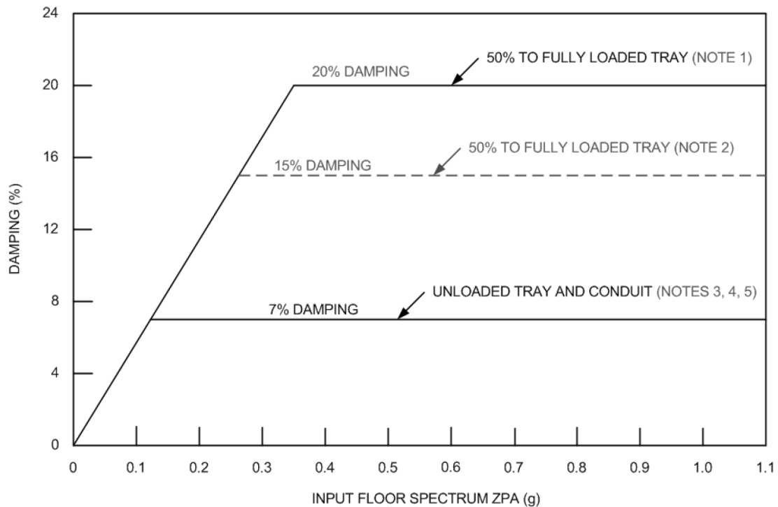
Figure 3.7.1-16—Damping Values for Cable Trays with Flexible Support Systems
