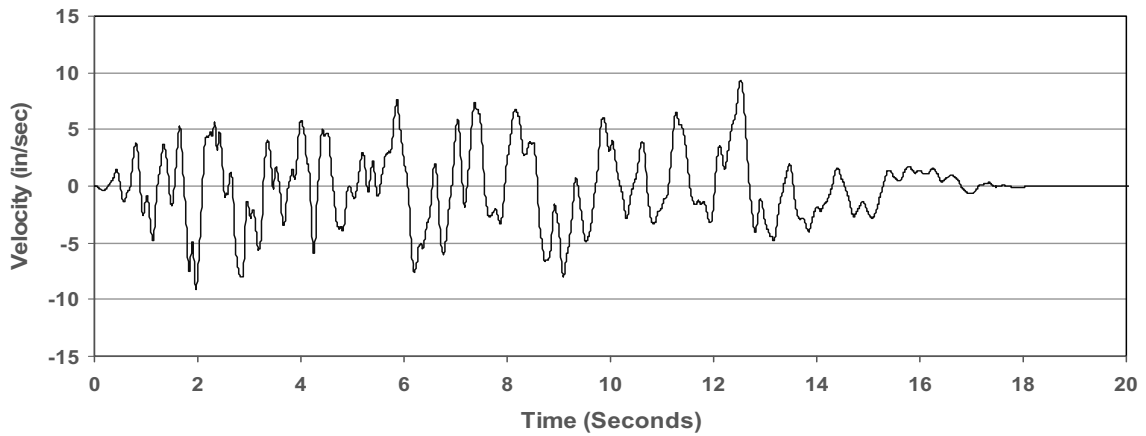
EURS3 - INTEGRATED VELOCITY TIME HISTORY
