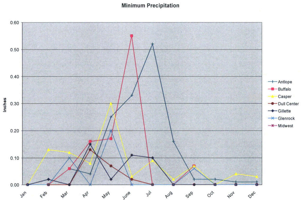
Figure 3-4c Monthly Minimum Precipitation (in inches) for Select Stations.
