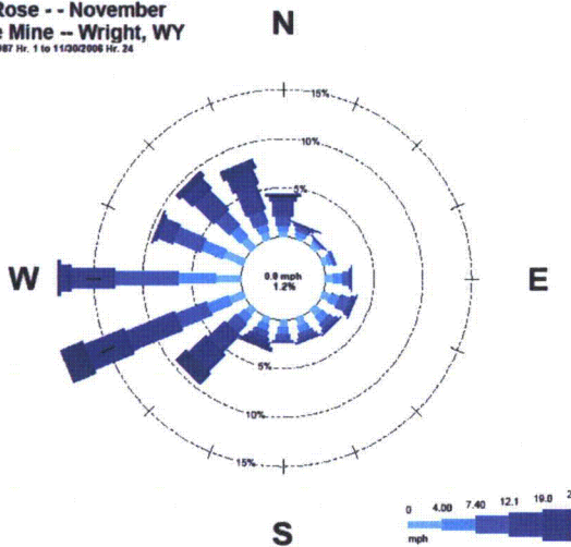
Wind Rose - - December Antelope Mine - - Wright, WY 12/1/1987 Hr. 1 to 120312006 Hr. 24
