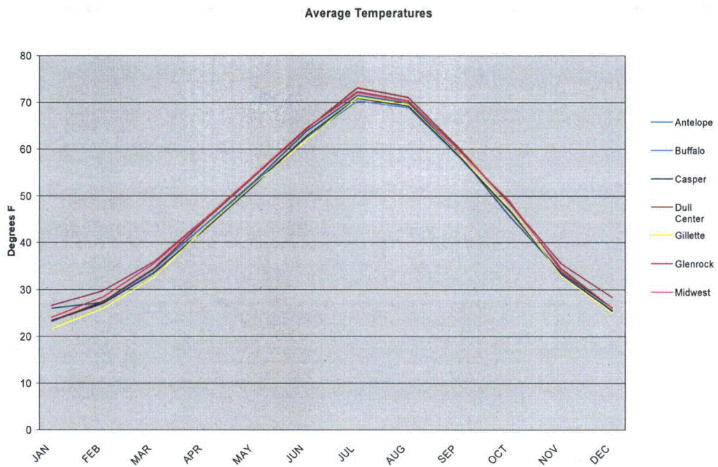
Figure 3-2 Average Monthly Temperatures for Select Meteorological Stations.
