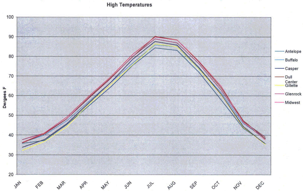
Figure 3-4 Average Monthly Maximum Temperatures for Select Meteorological Stations.
