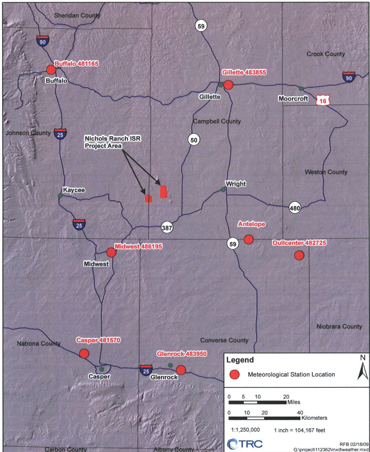
Figure 3-1 Location of Regional Meteorological Stations.
