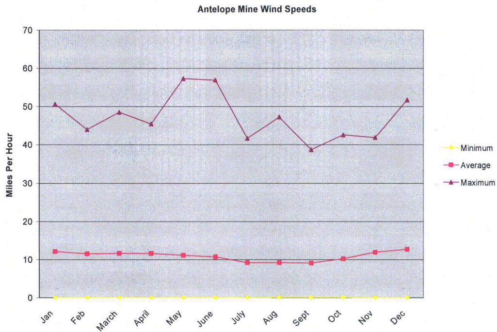
Figure 3-4e Average Monthly Wind Speeds (mph) at the Antelope Station.
