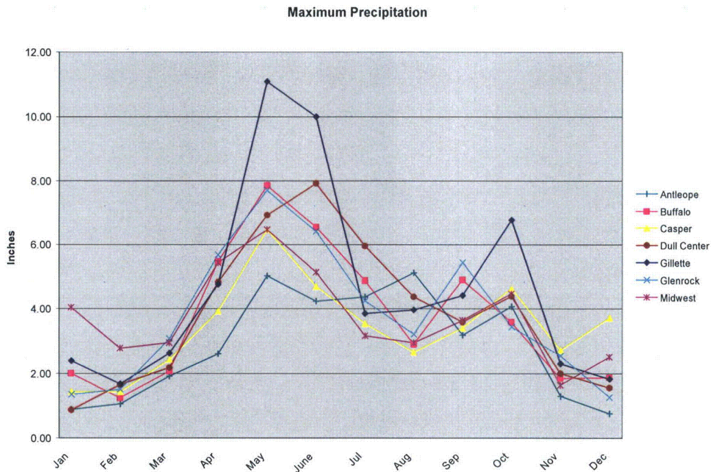
Figure 3-4d Monthly Maximum Precipitation (in inches) for Select Stations.
