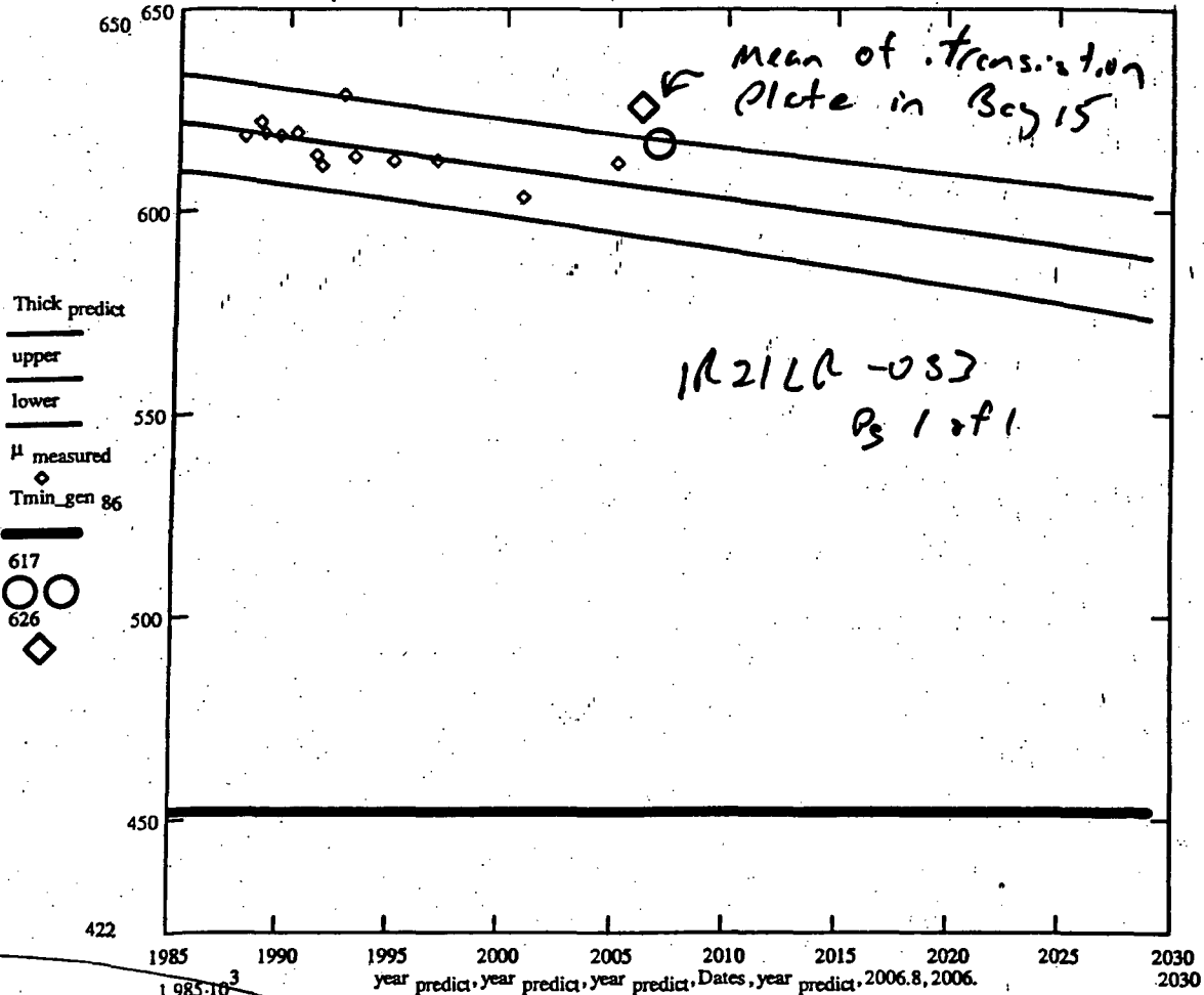
Location Curve Fit Projected to Plant End Of Life
