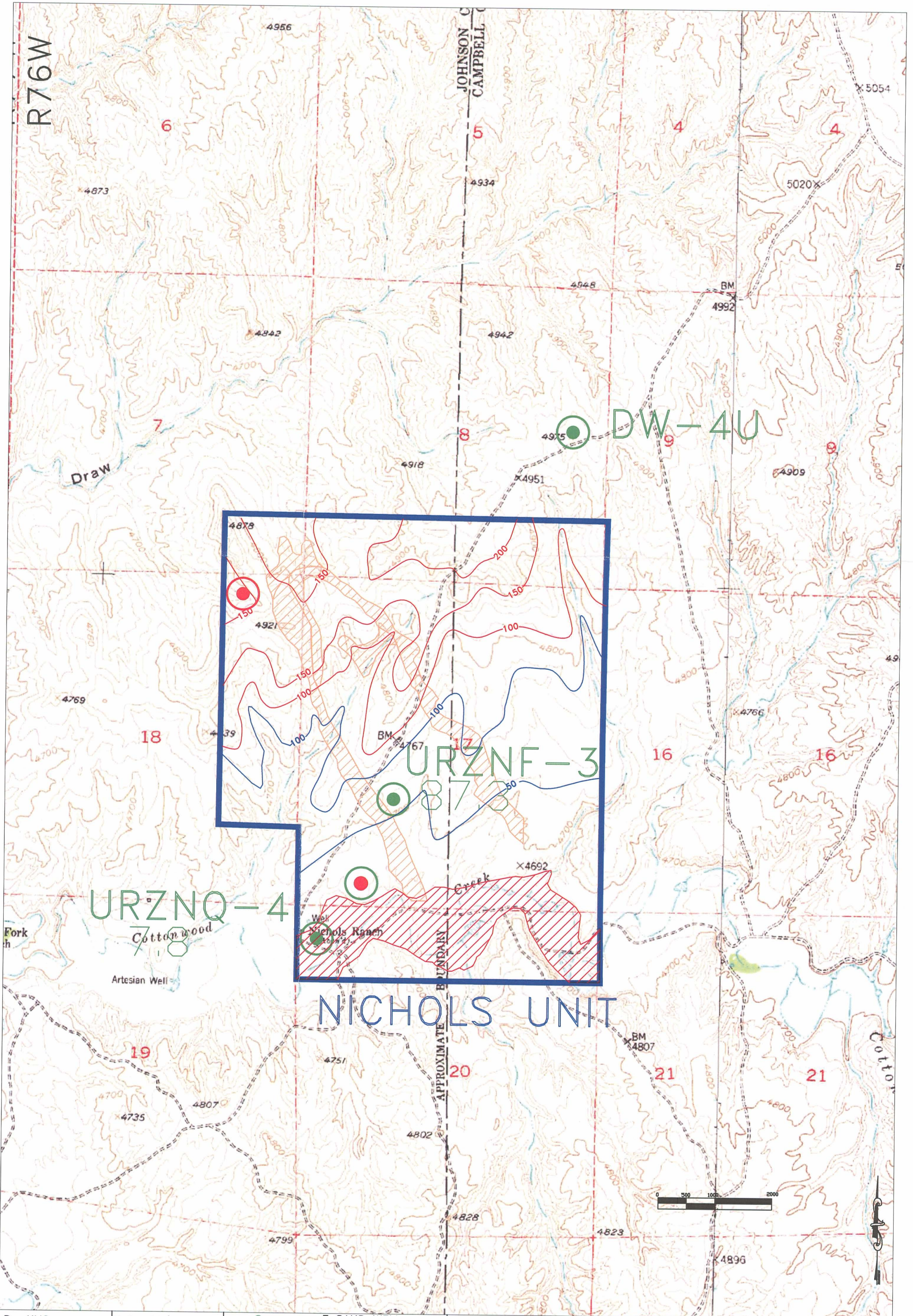
FIGURE 2-21a. DEPTH TO WATER IN THE F & G SANDS AND COTTONWOOD ALLUVIAL AT THE NICHOLS RANCH UNIT, IN FT
