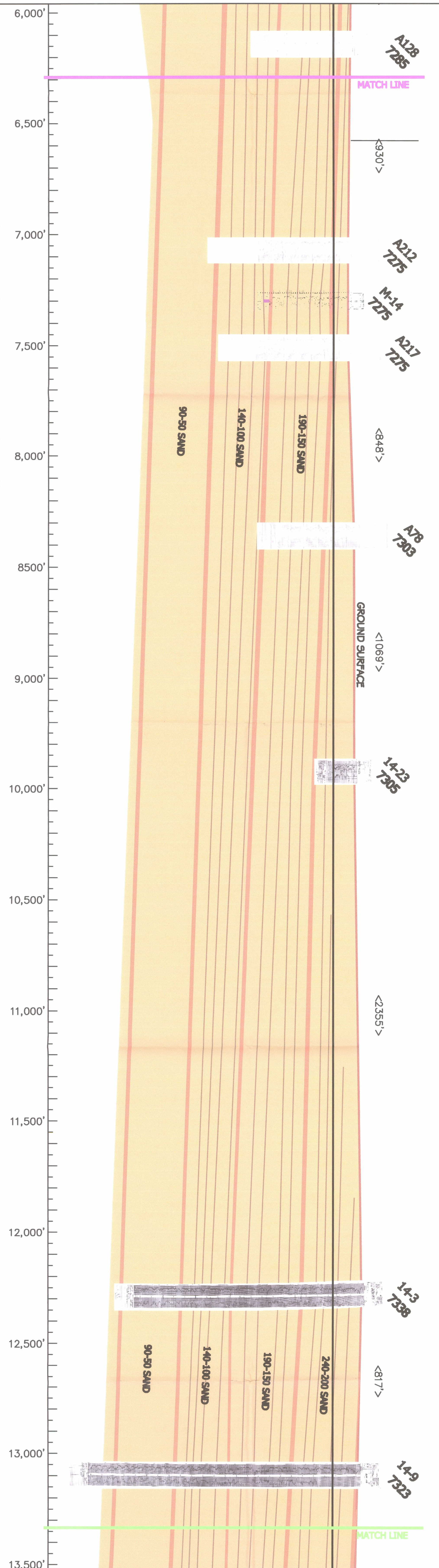
STRATIGRAPHIC CROSS SECTION S7-S7' FIGURE 2.6-28A
