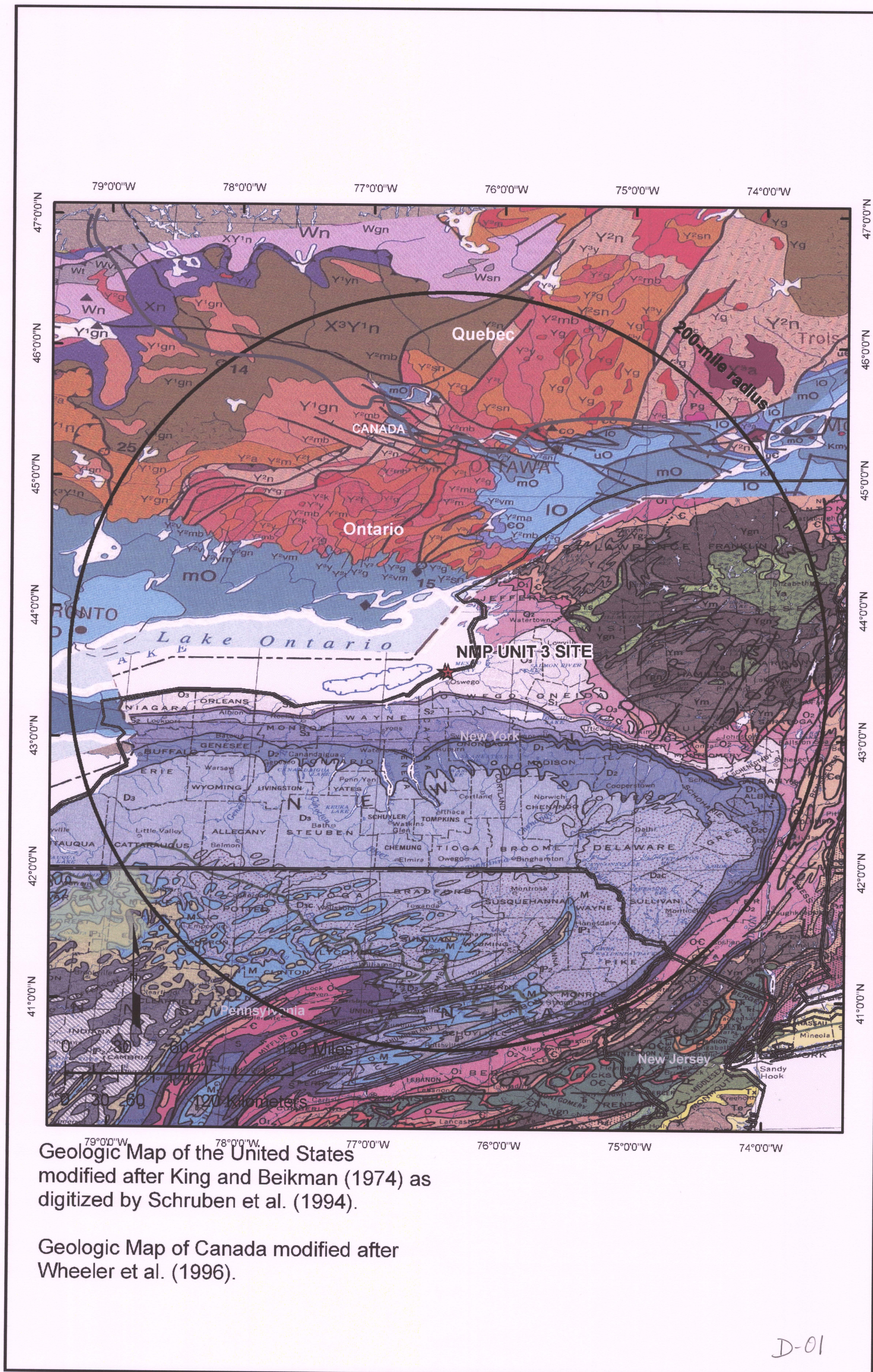
Figure 2.5-2—{Regional Geologic Map}
