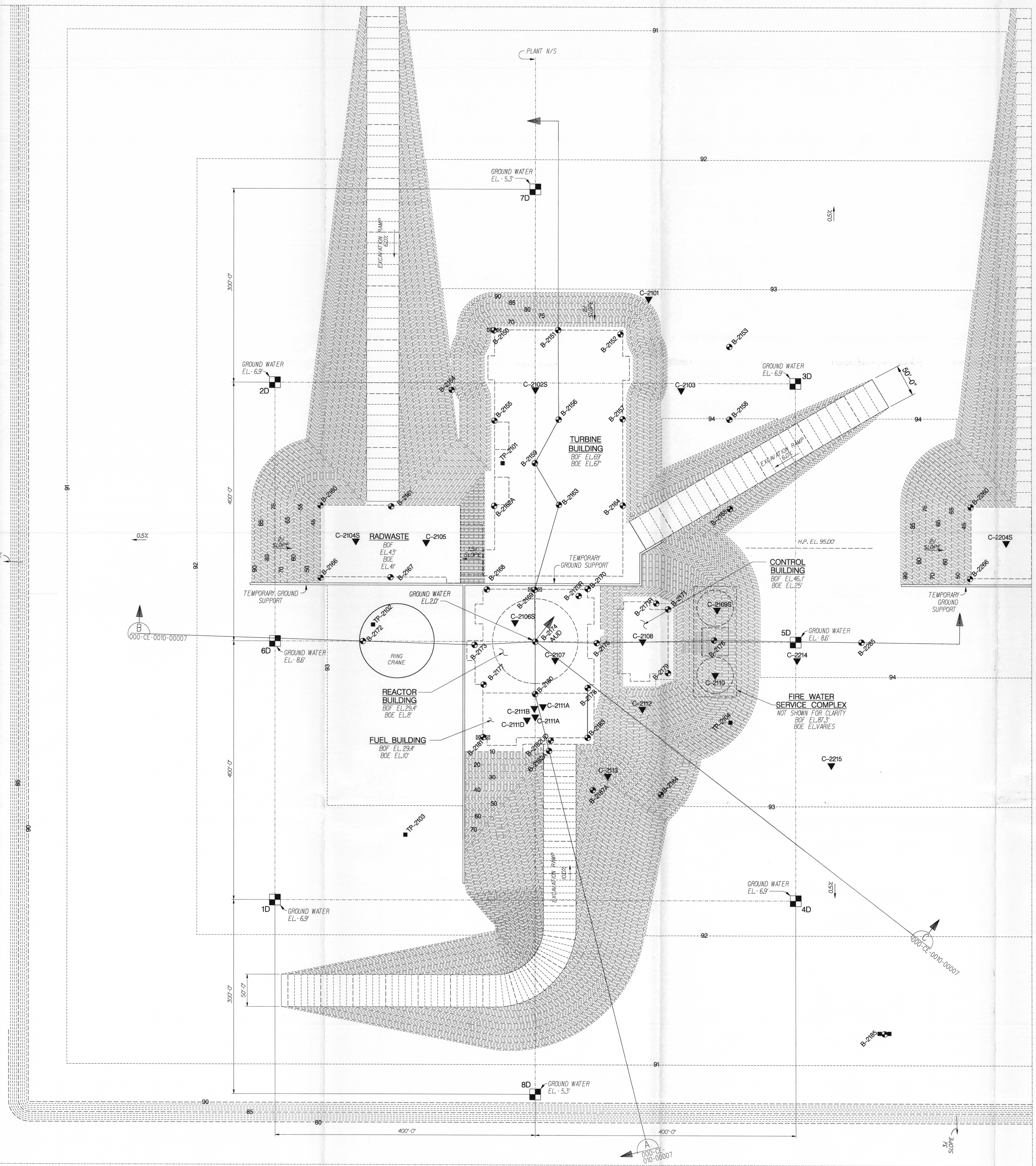
FIGURE 3 - DEWATERING PLAN, DEEP AQUIFER
