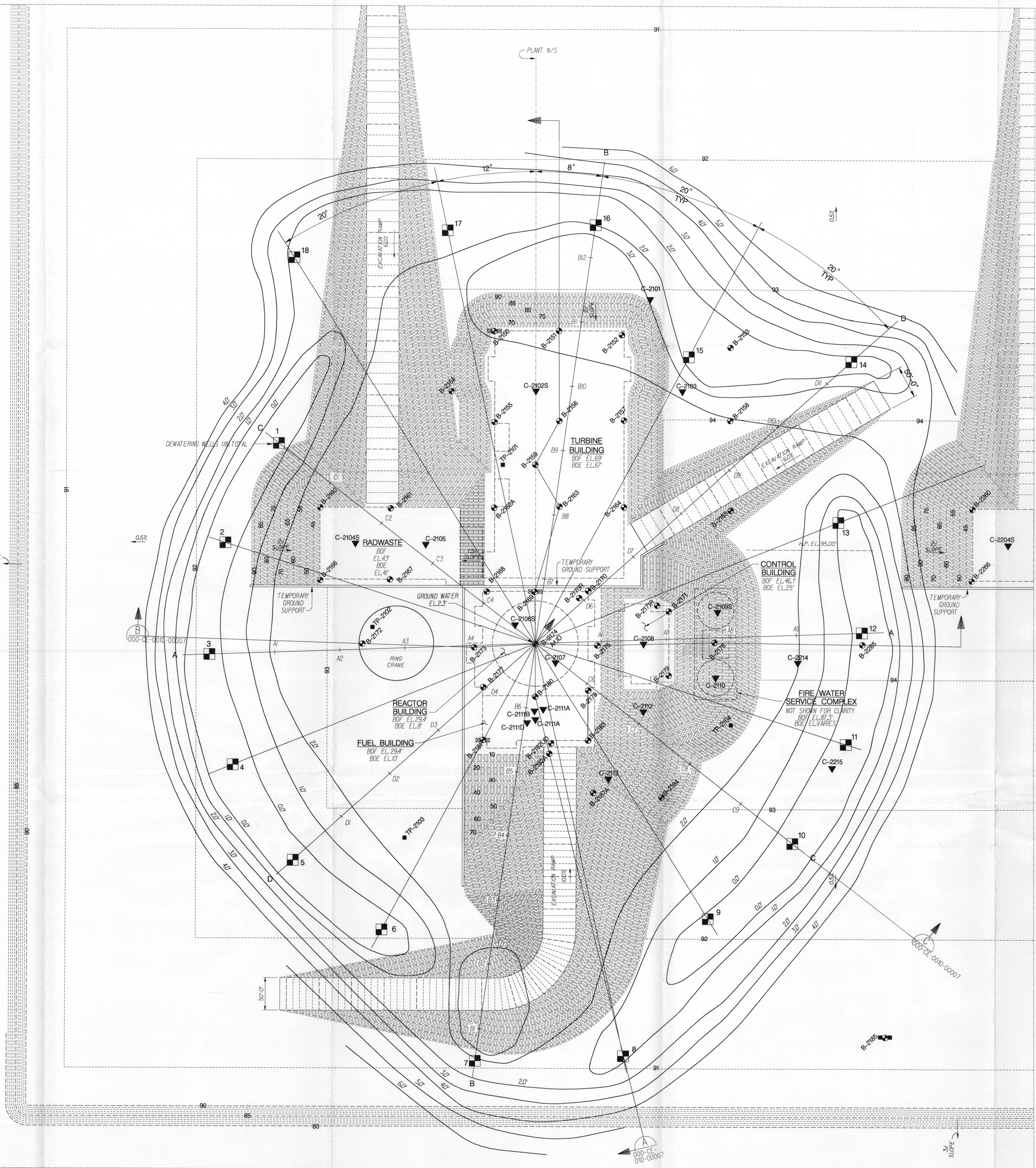
FIGURE 1 - DEWATERING PLAN
