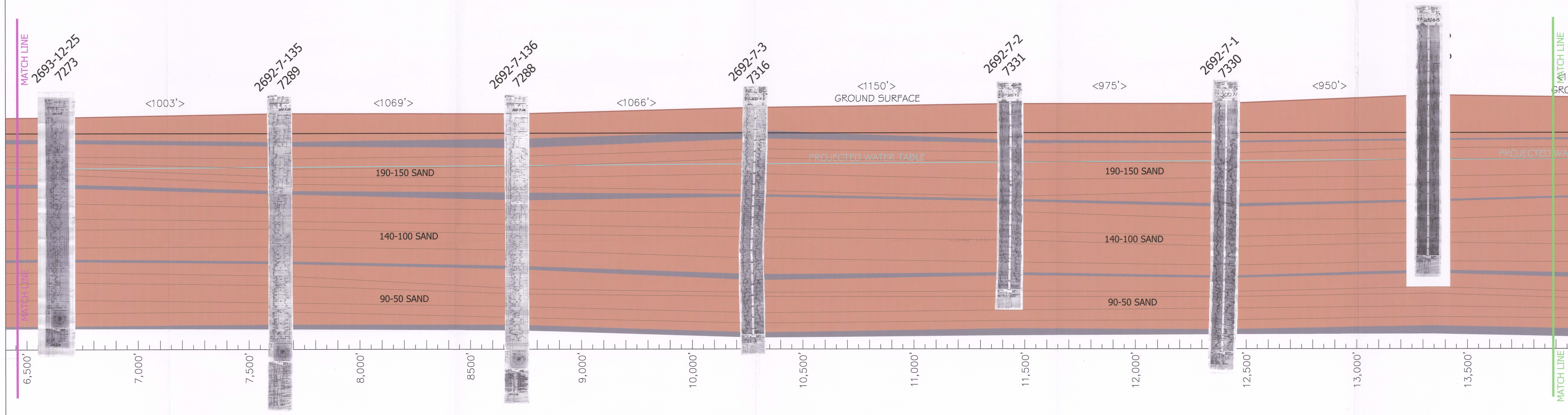
STRATIGRAPHIC CROSS SECTION L1-L1' FIGURE 3.3-25A
