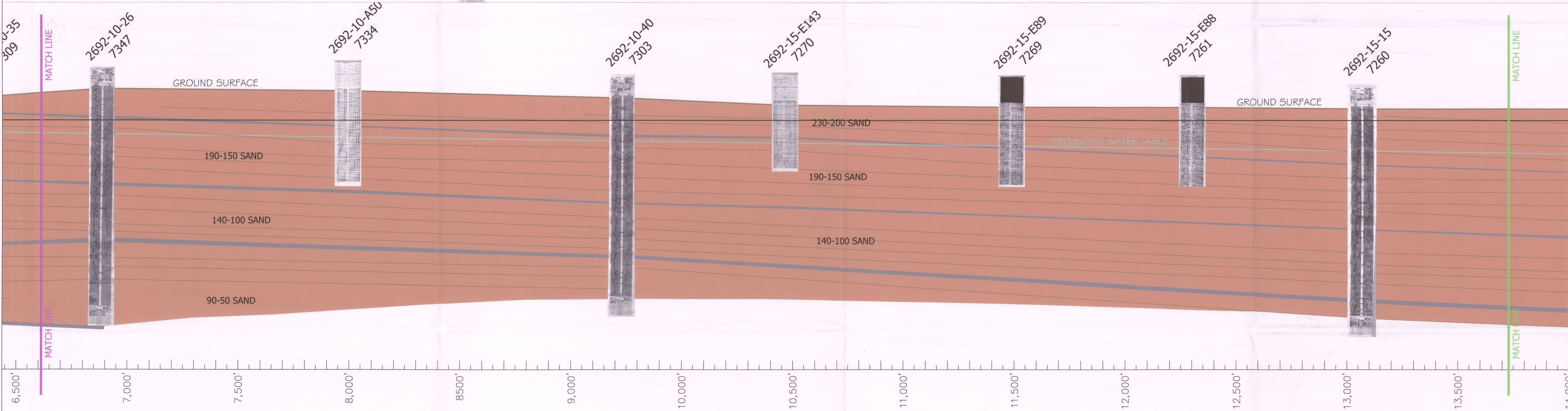
STRATIGRAPHIC CROSS SECTION S8-S8' FIGURE 2.6-29A
